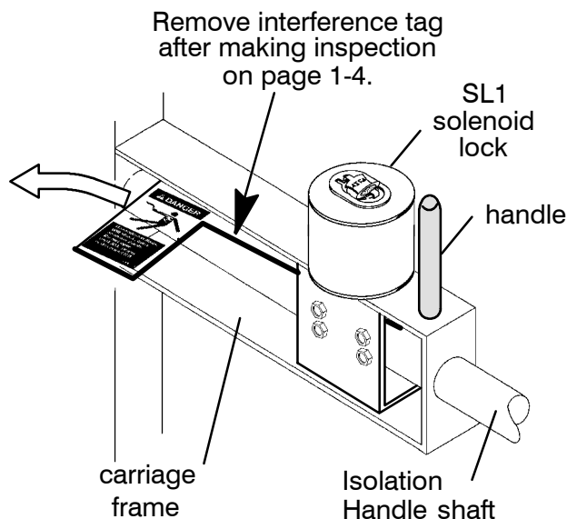
Figure 1-2. Solenoid latch interference tag.
