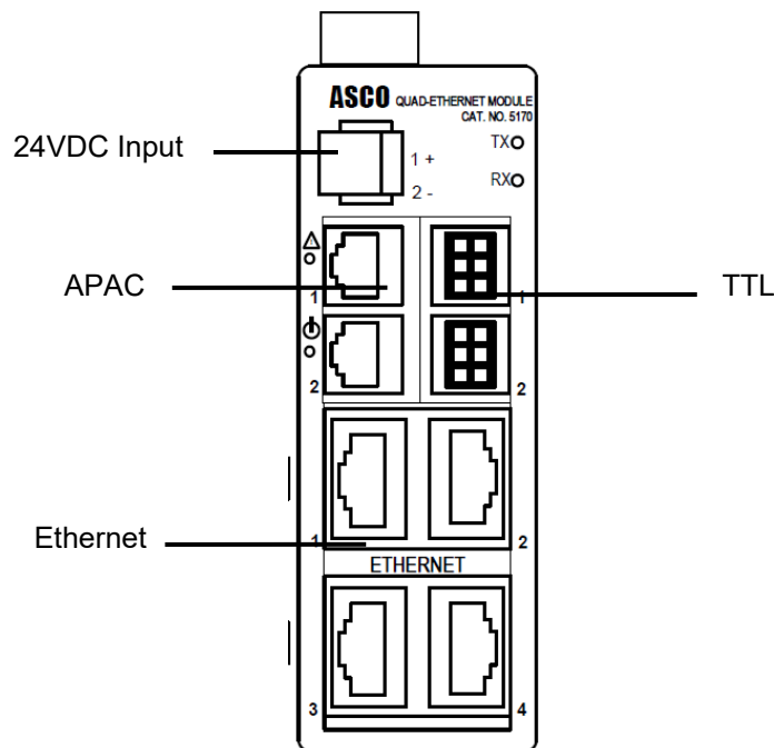
Figure 2. Ethernet an Operational Power Connections
