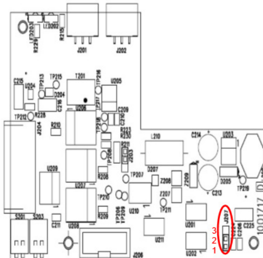
Figure 48. New location of jumper pins
