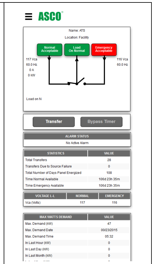
Figure 10. Mobile Device View Dashboard page
