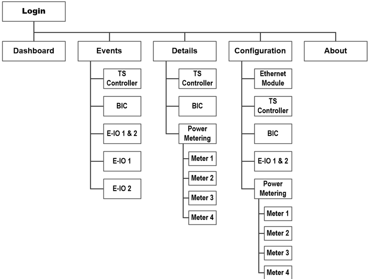
Figure 11. Navigation Menu-bar and drop-down boxes.
