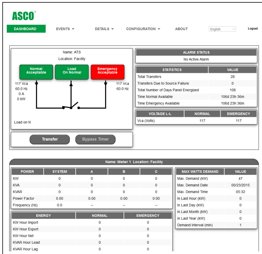
Figure 9. Desktop View Dashboard page
