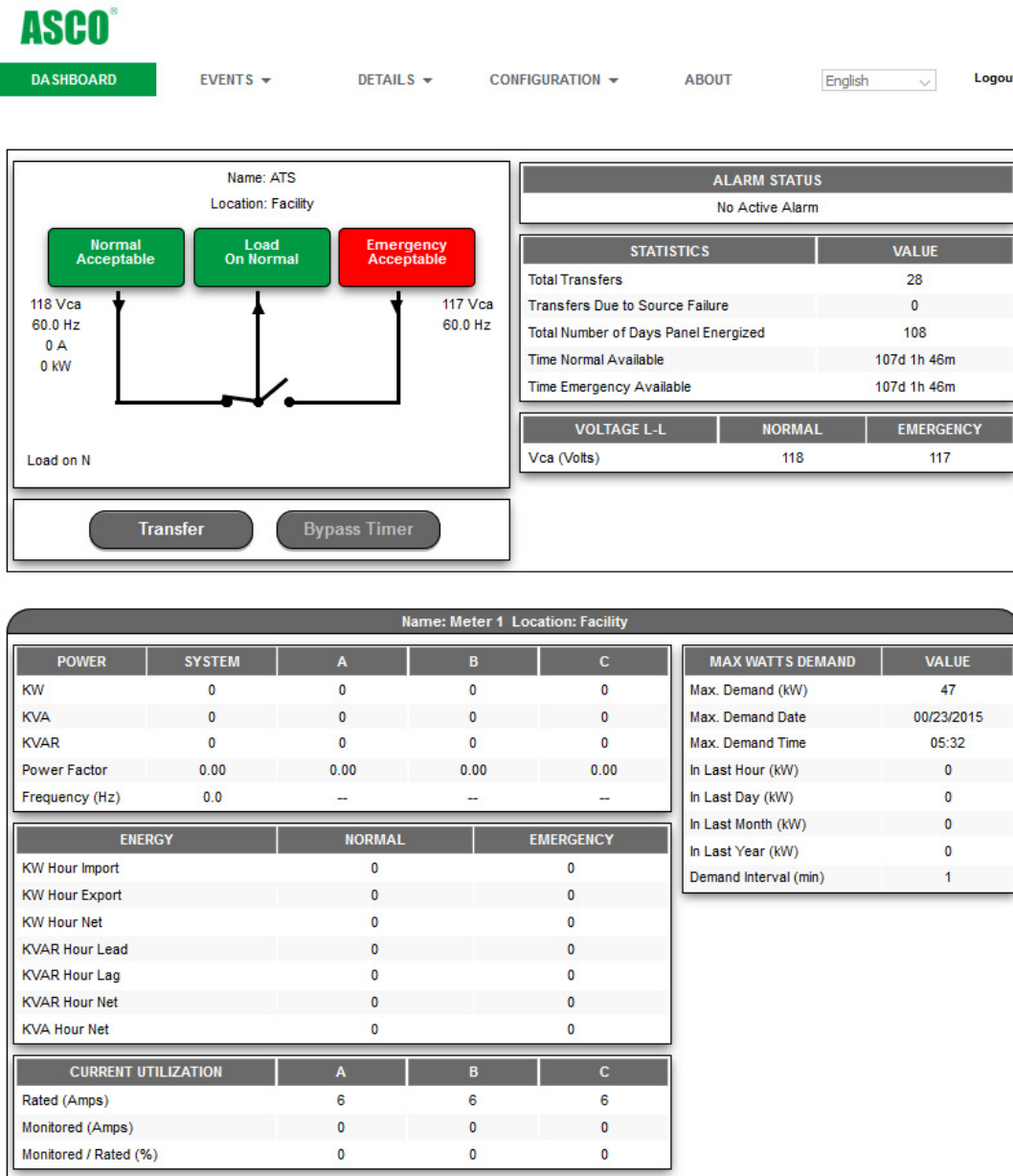
Figure 45. Dashboard Screen Group 5 Controller with a single Power Meter
