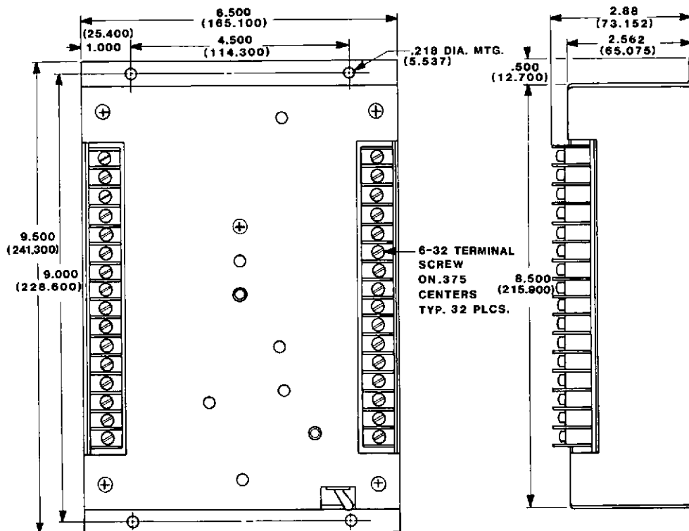
FIGURE 18 — OUTLINE DRAWING
