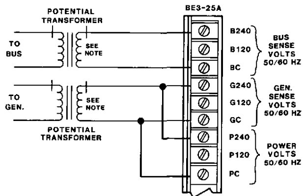
FIGURE 17 -- 240 VAC, POWER FROM GENERATOR
