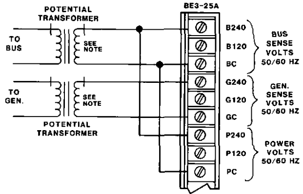
FIGURE 15 -- 240 VAC, POWER FROM BUS
