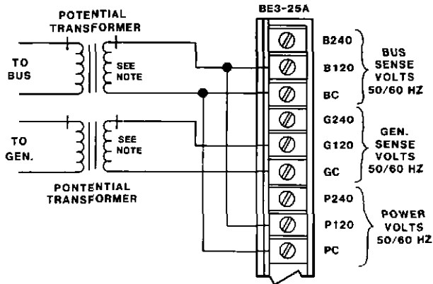
FIGURE 14 -- 120 VAC, POWER FROM BUS
