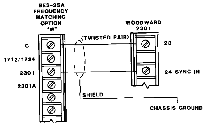
FIGURE 5 – WOODWARD 2301 INTERCONNECTION
