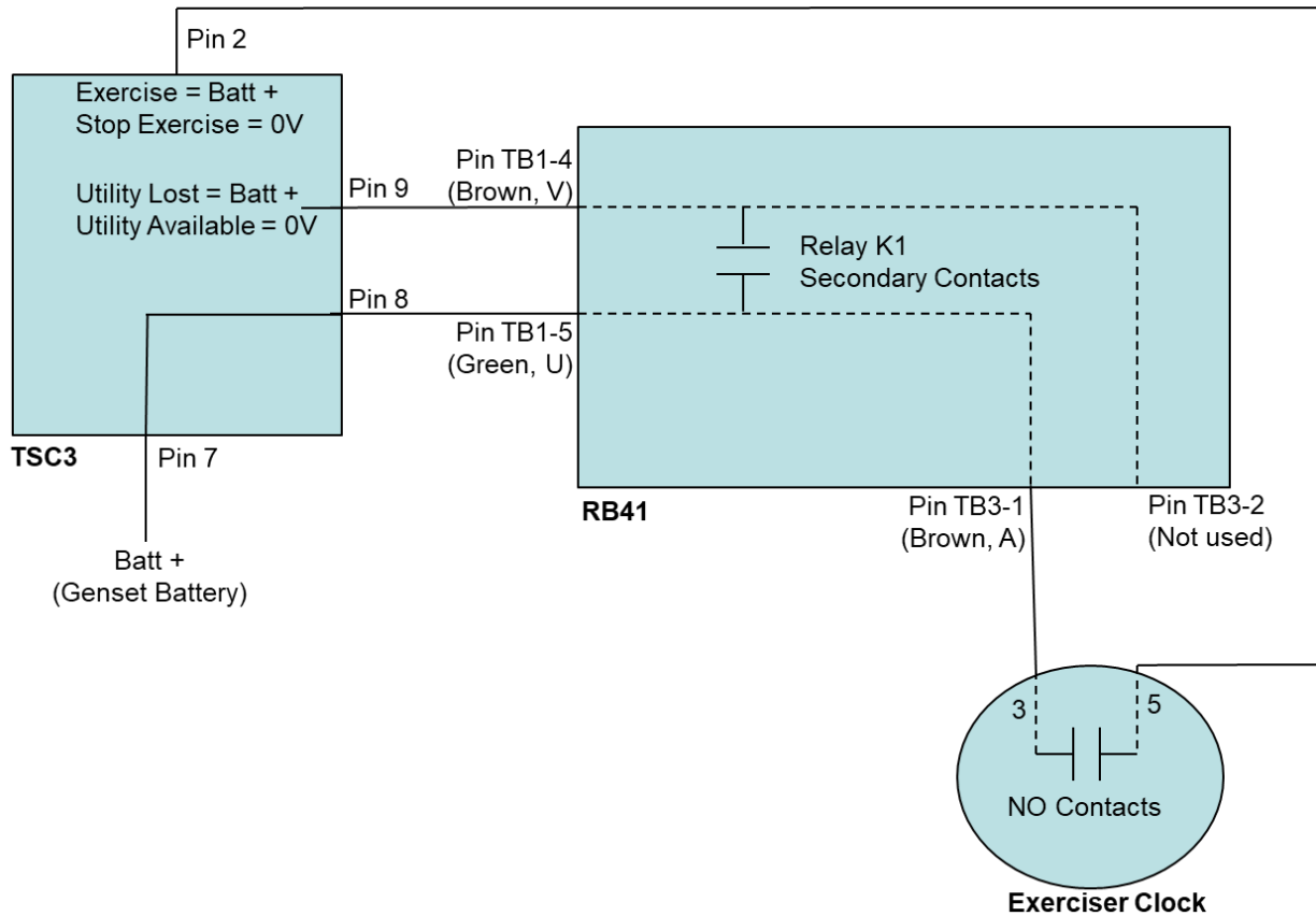
Figure 5 – OPT Transfer Switch RB41 control logic
