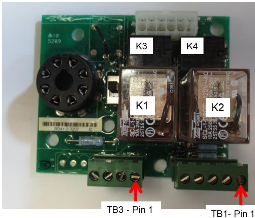
Figure 2 – RB41 Pinout
