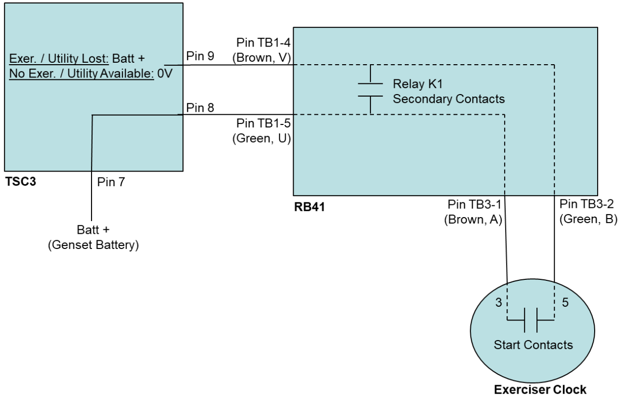
Figure 4 – AST Transfer Switch RB41 control logic
