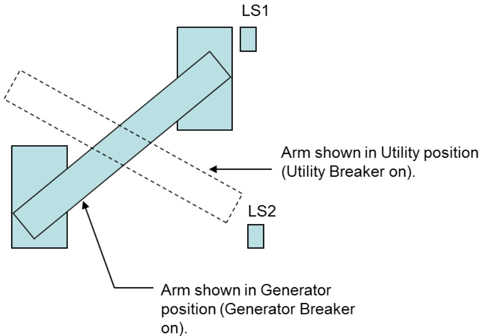
Figure 1 – AST/OPT Transfer Arm
