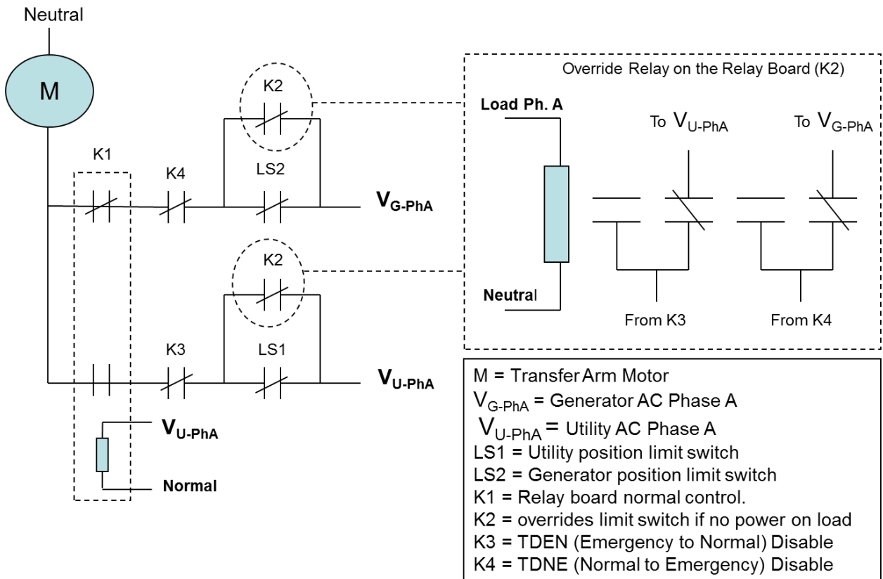
Figure 3 – RB41 Motor Circuit
