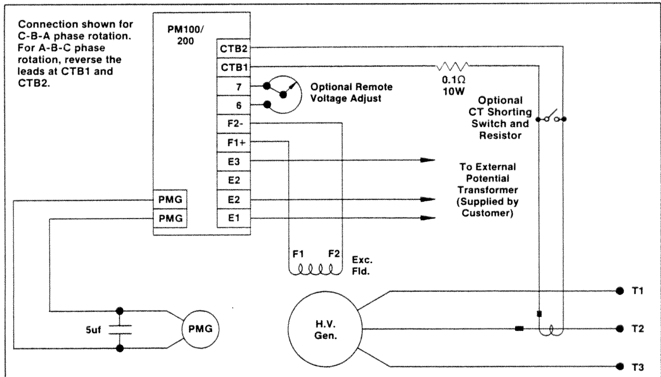
Typical Connection - Three Phase Sensing (601-6600 Volts) with Reactive Droop Paralleling
