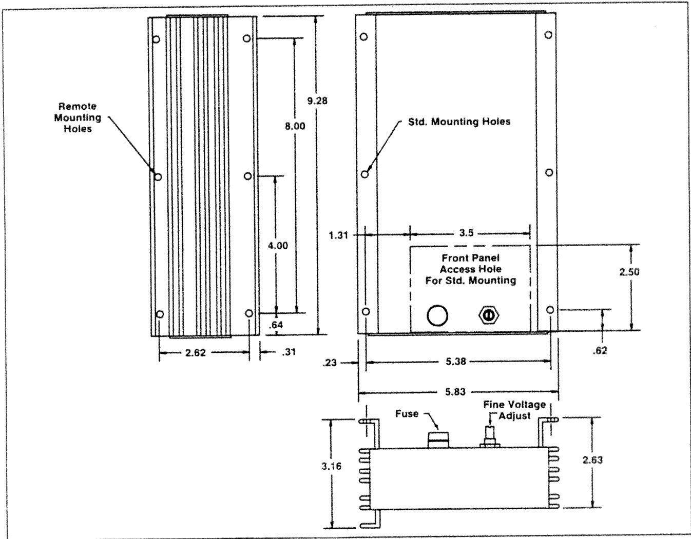
Outline Drawing of Regulator
