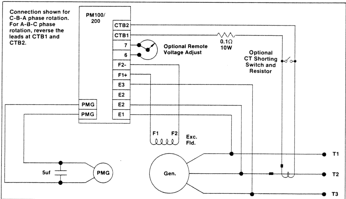
Typical Connection - Three Phase Sensing (95-600 Volts) with Reactive Droop Paralleling
