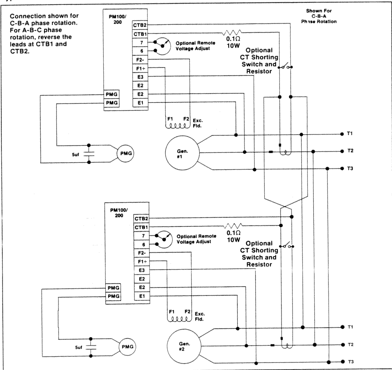
Typical Connection - Three Phase Sensing (95-600 Volts) with Reactive Differential Paralleling
