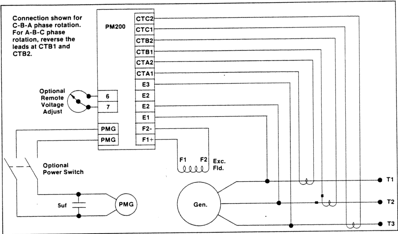
Typical Connection - Three Phase Sensing (95-600 Volts) with Generator Current Limit
