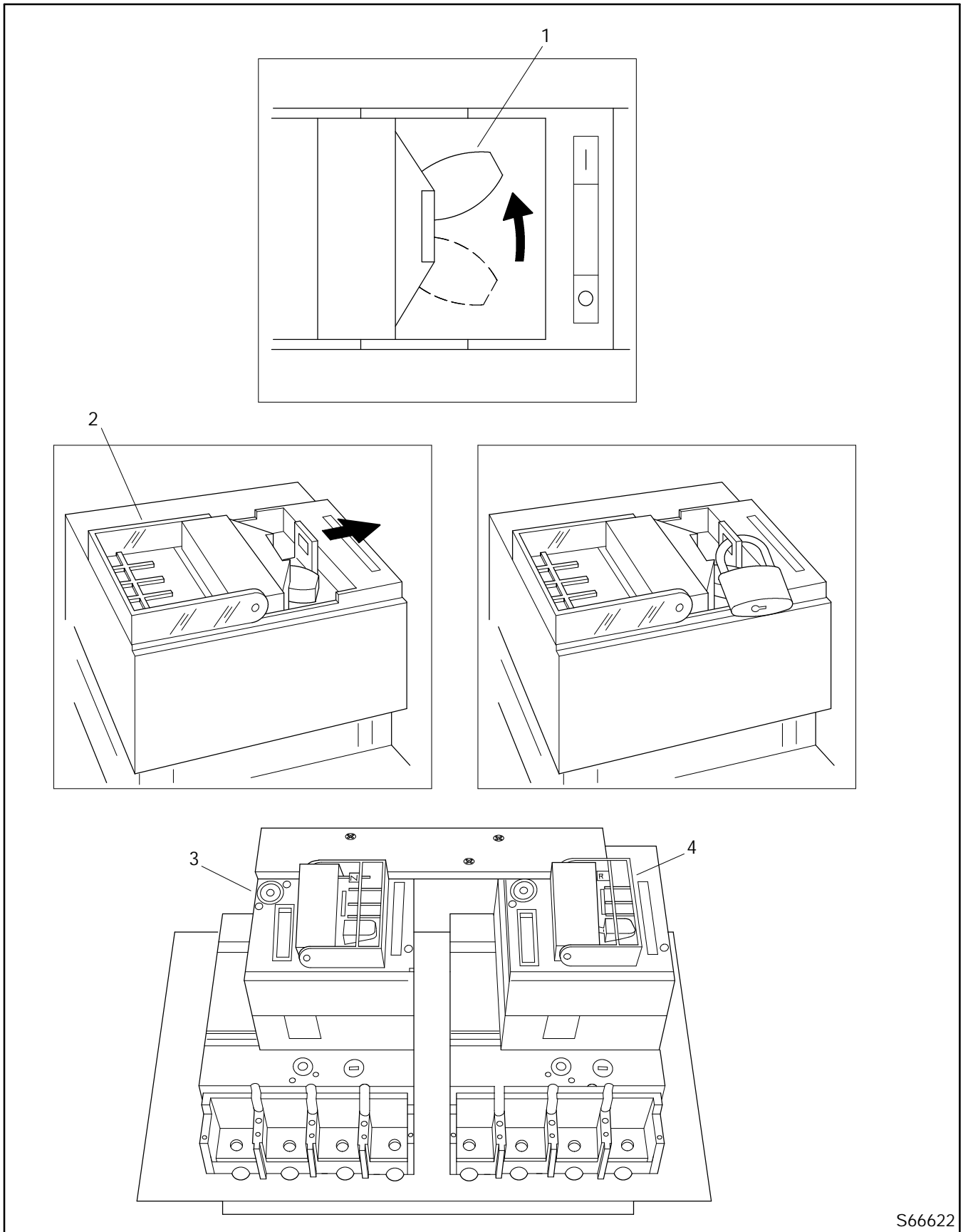
Figure 2-2. Automatic Transfer Switch (250-1250 Ampere) Operation
