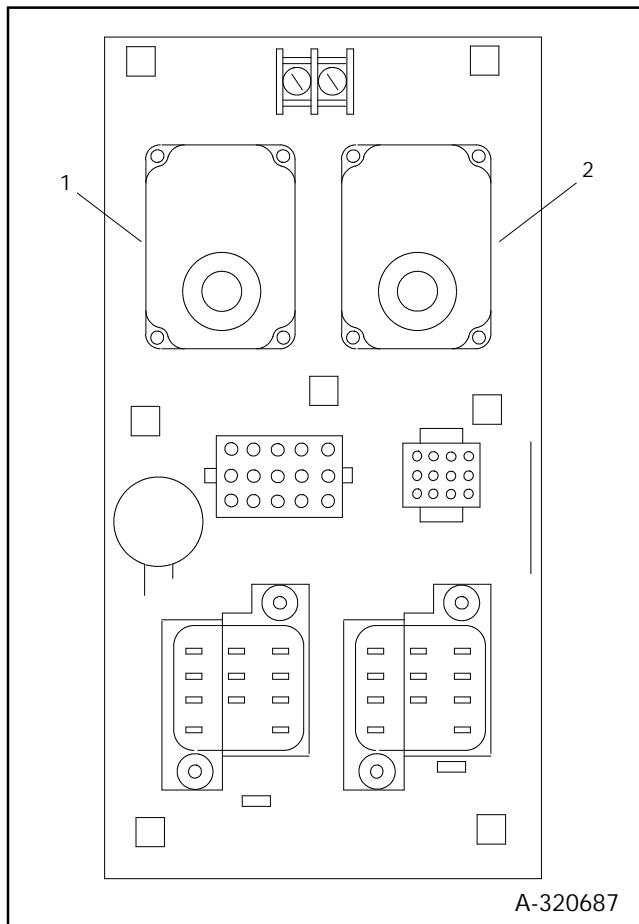
Figure 2-5. Interface Board with Time Delay Relays
