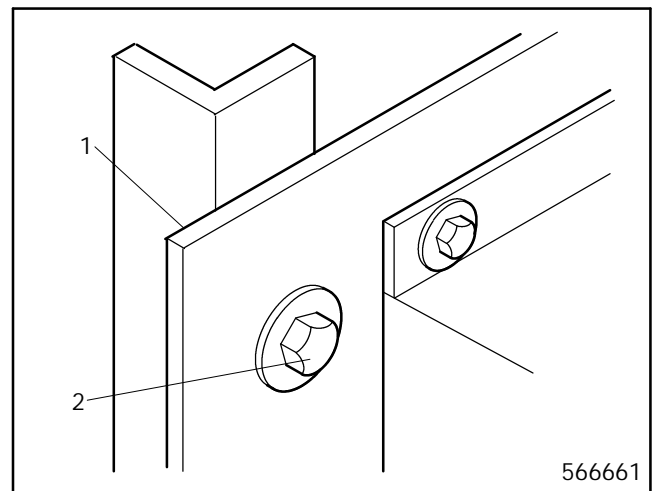
1 Contactor Assembly 2 Screw and Washer
