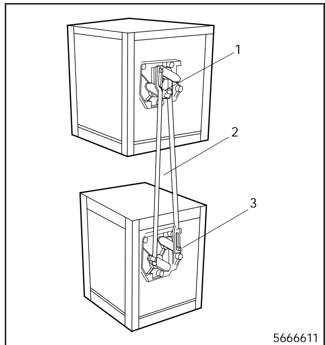
Figure 6-11. Mechanical Interlock Rod Removal
