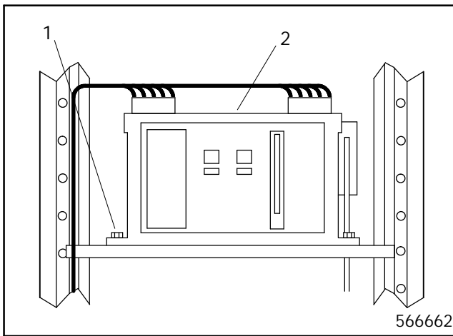
1. Mounting Hardware 2. Contactor
