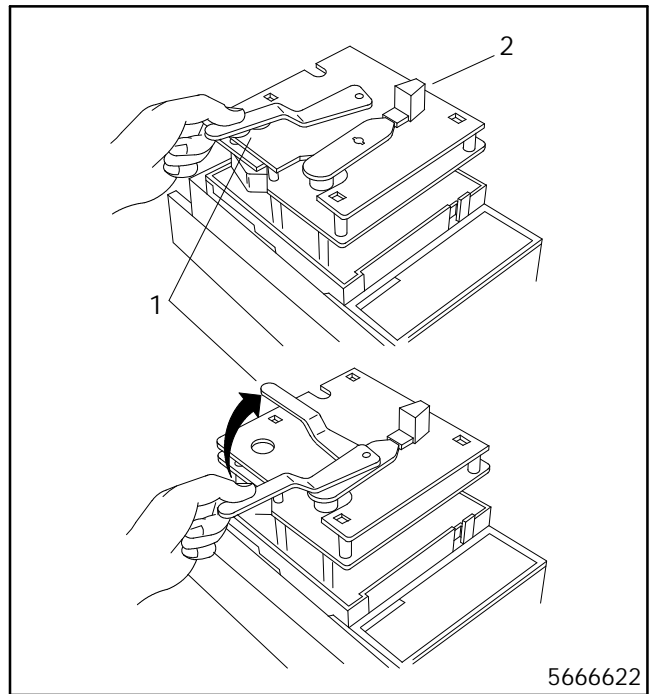
Figure 6-22. Install Interlock Control Arm
