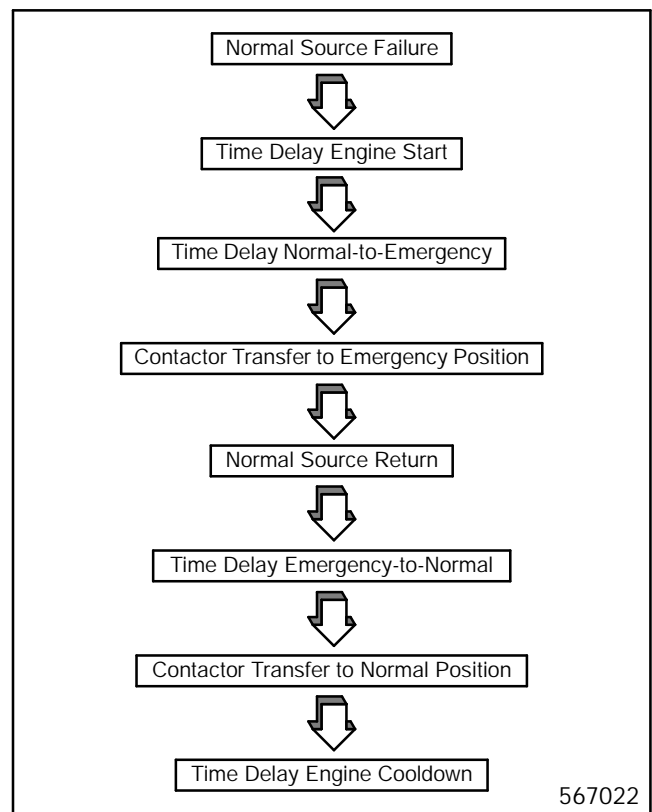
Figure 2-4. Logic Board Operation
