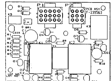
CONTROL BOARD
