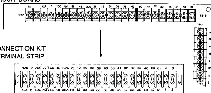
DECISION MAKER CIRCUIT BOARD
