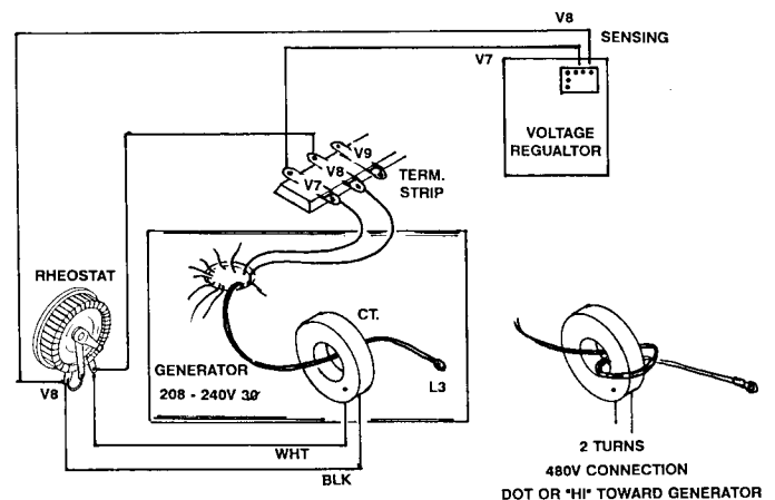
TYPICAL FR11 KIT CONNECTION
