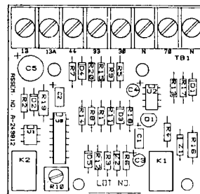
OVERSPEED/TD BOARD
