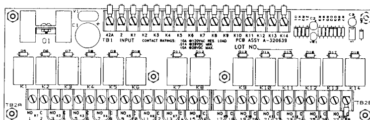
DRY RELAY CONTACT KIT
