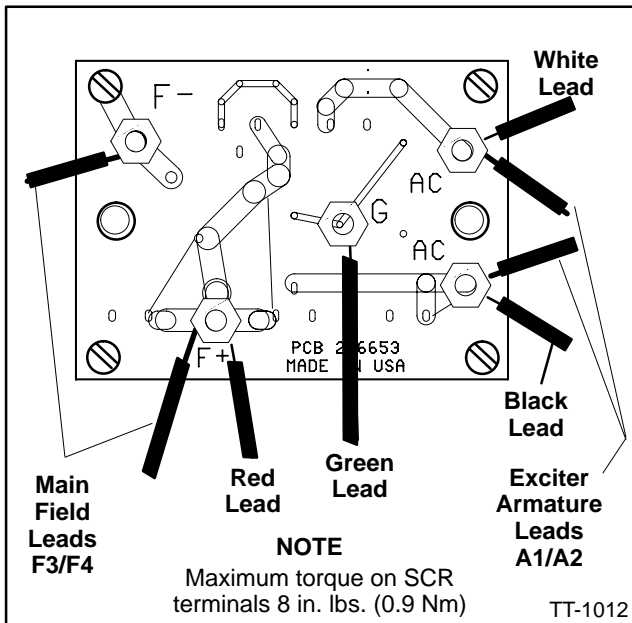
Figure 4. SCR Assembly Wiring
