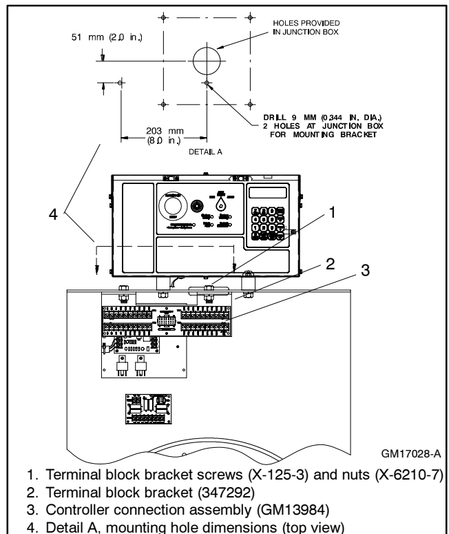
Figure 3 Terminal Block Bracket and Controller Connection Assembly Mounting (350/400 kW)
