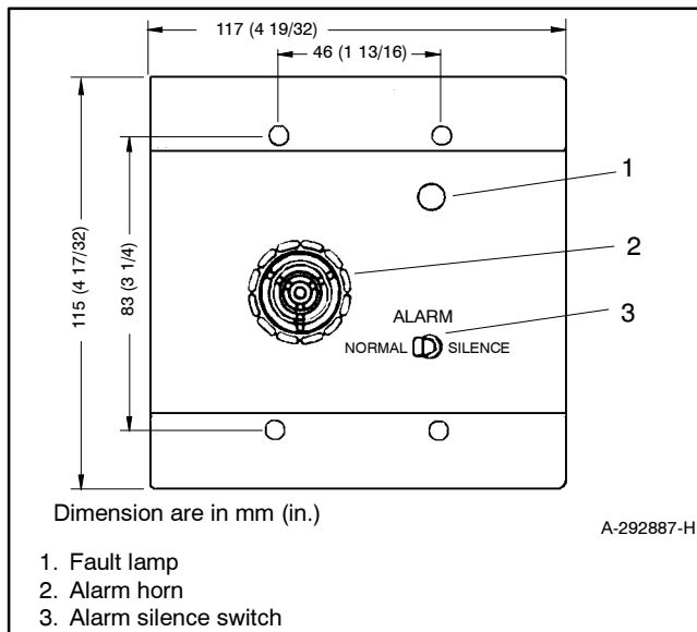
Figure 1 Audiovisual Alarm Panel
