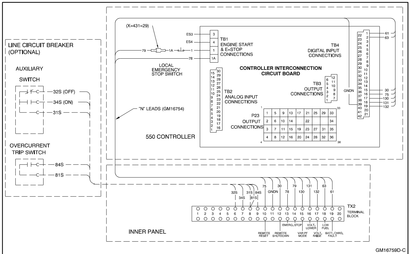
Figure 6 Attaching Wiring Connection Harness to TX2 Terminal Block
