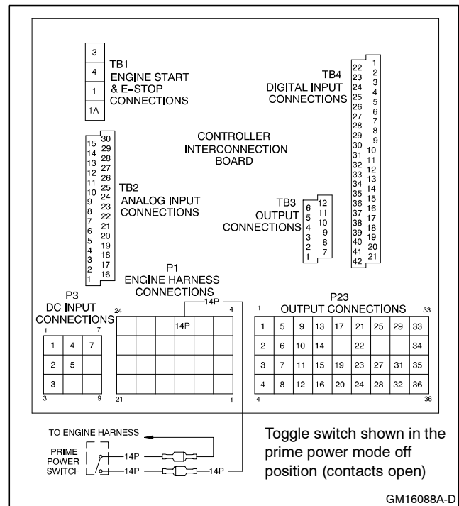
Figure 2 Toggle (Prime Power) Switch Connections
