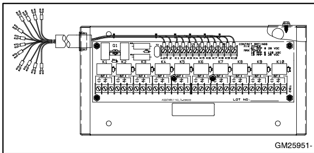
Figure 1 Ten-Relay Dry Contact Kit (20-400 kW Model kit shown)
