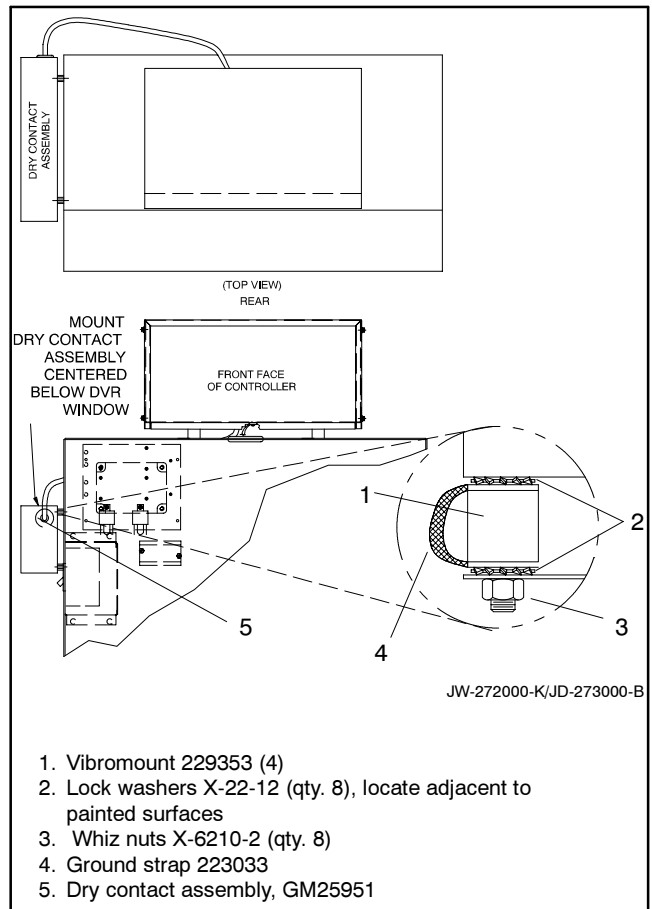
Figure 8 Junction Box Drilling Information (350/400 kW)
