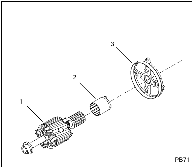
Figure 1. Alternator Components
