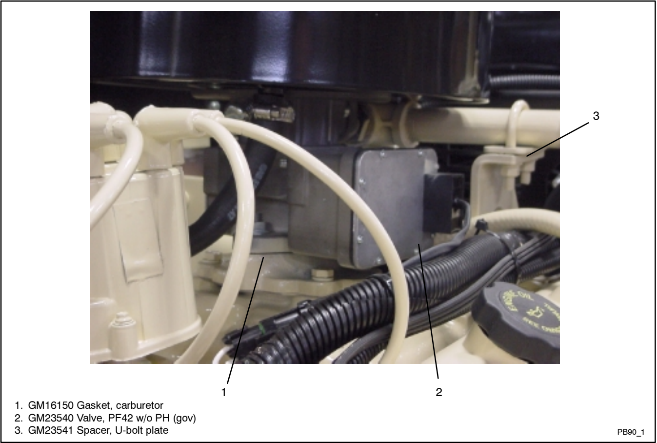
Figure 1 Kit GM23538 for 4.3 L Engine (continued)
