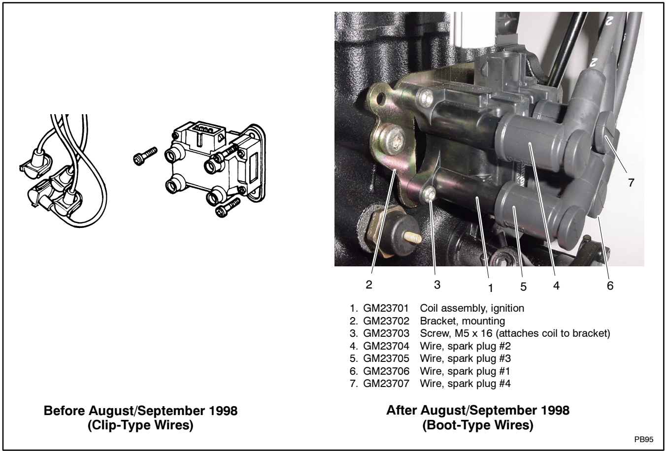
Figure 1 Ford VSG-413 Ignition Coil and Spark Plug Wires
