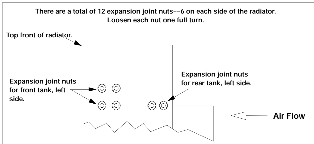
Figure 1. Expansion joint nuts, top left side of radiator (typical).
