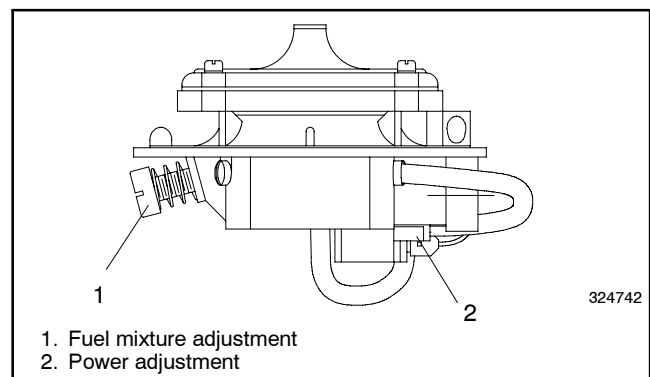
Figure 9 30-80 kW with Nolf NCA-225M and NCA-125M Style Fuel Mixers
