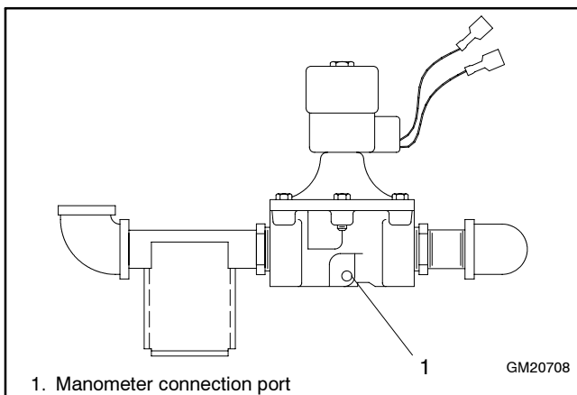
Figure 5 Solenoid Fuel Valve Manometer Port
