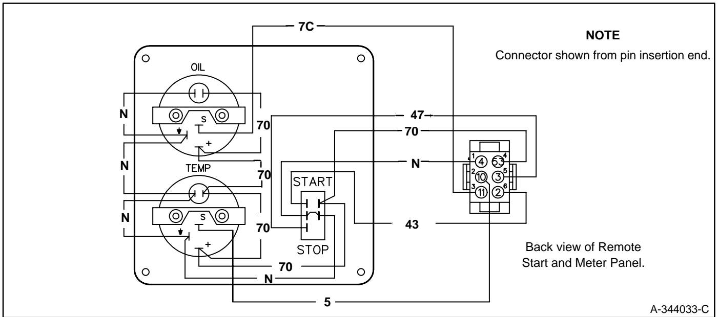
Figure 3. Typical Electrical Connections
