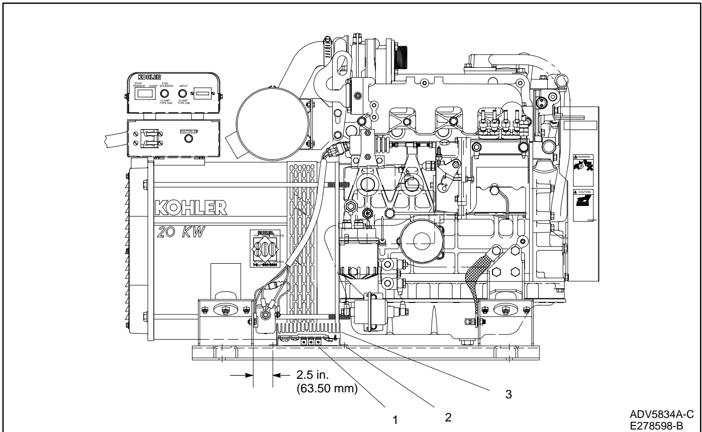
Figure 1. Voltage Regulator Mounting Installation
