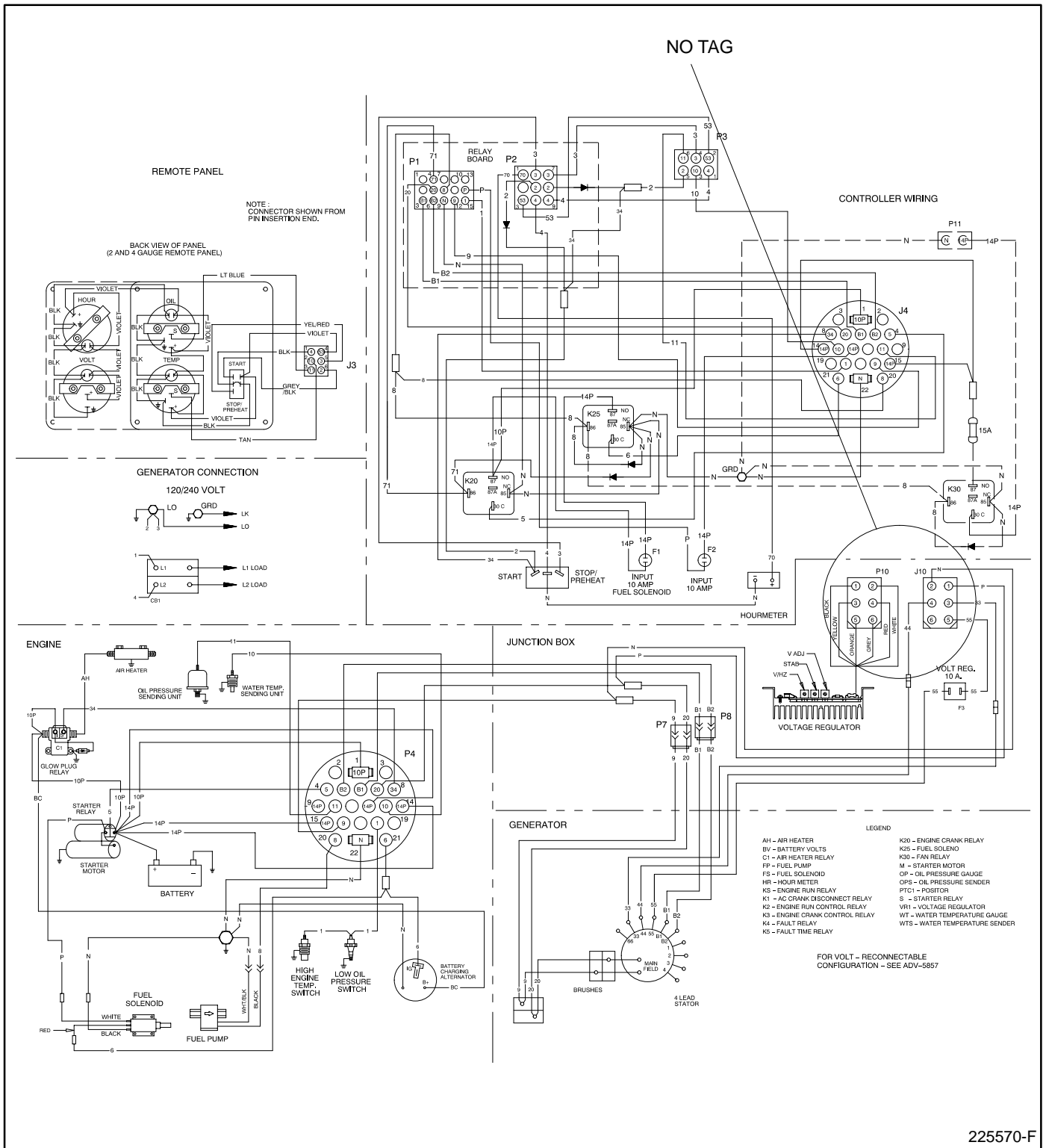
Figure 2. Wiring Diagram
