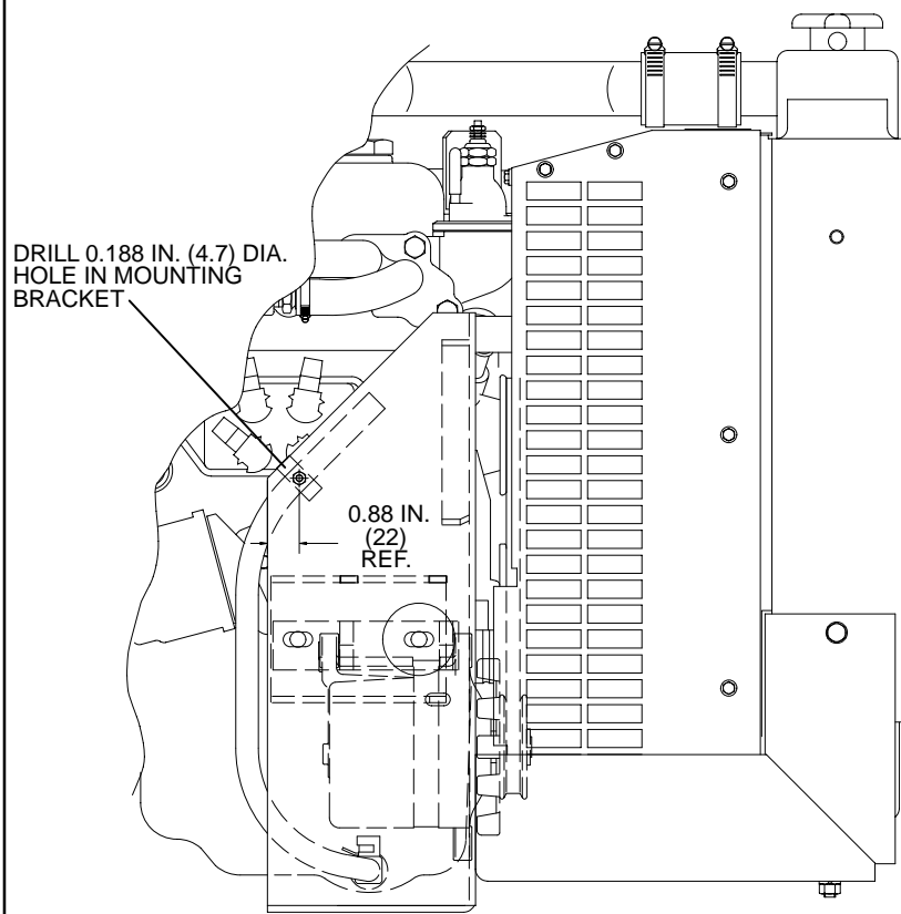
Figure 1. Installing Kit
