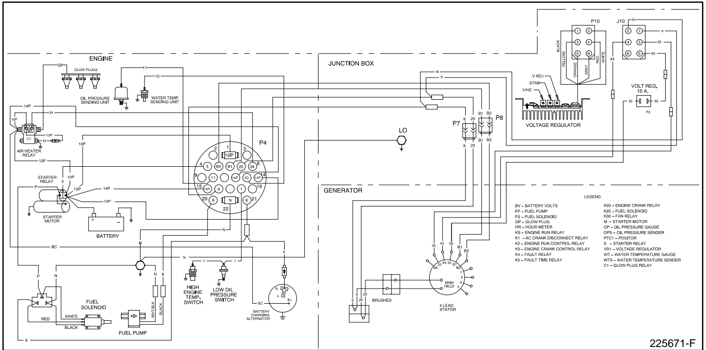
Figure 2. Wiring Diagram of 225671
