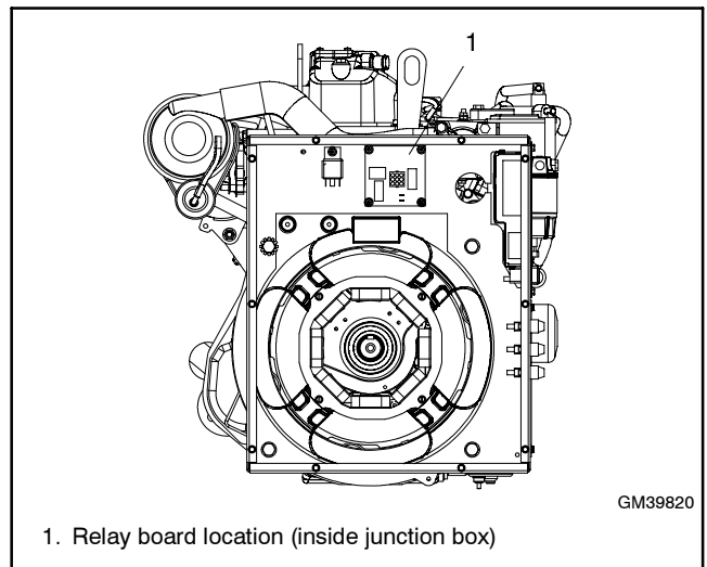
Figure 3 Relay Board Location, Models 10/15/20REOD/REOZD/EORD/EORZD
