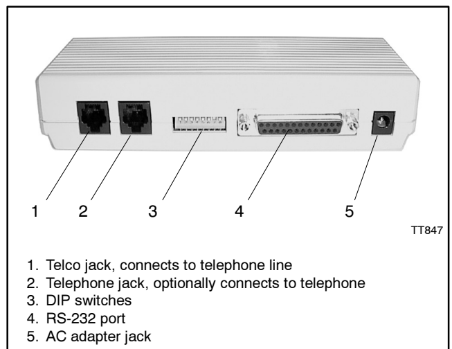
Figure 8 External Modem (typical), Rear View
