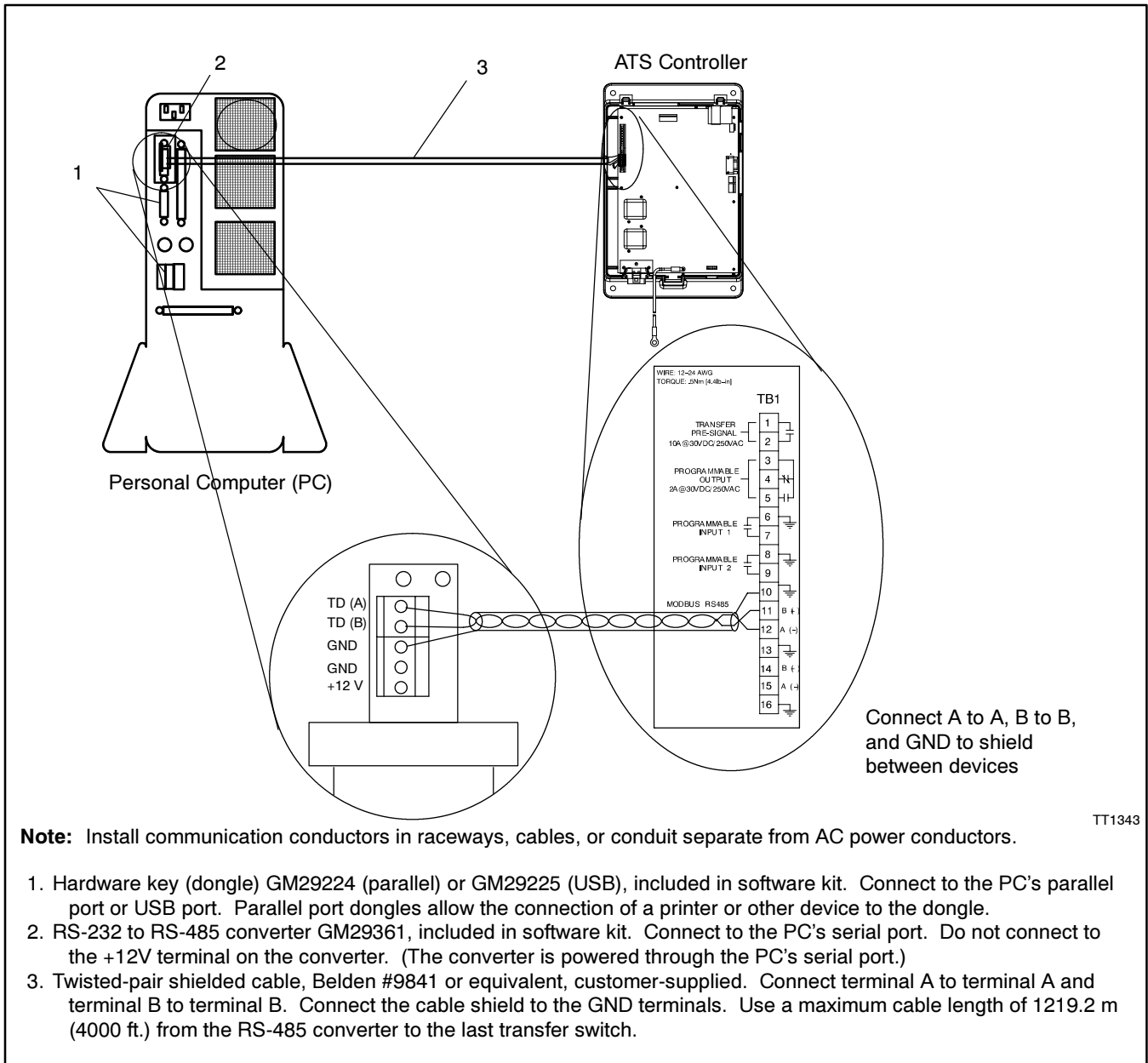
Figure 9 Local Single Connection Up to 1219.2 m (4000 ft.)
