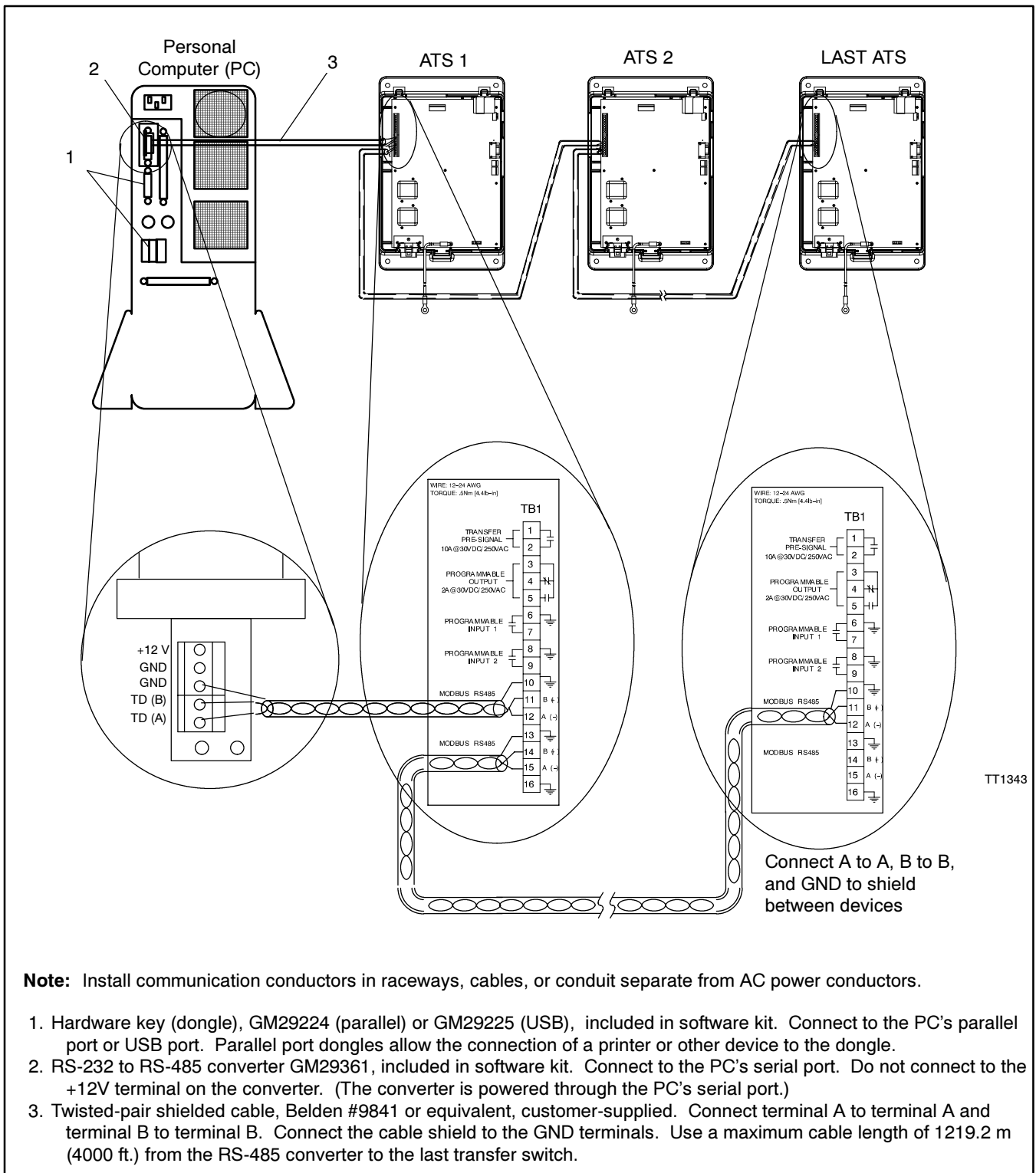
Figure 10 Local Area Network
