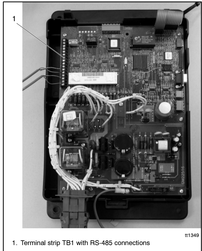
Figure 1 ATS Controller (cover removed)
