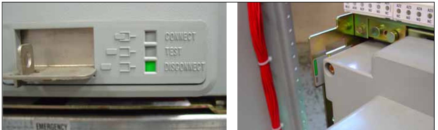
Figure 31. Switching Device in the DISCONNECT Position.
