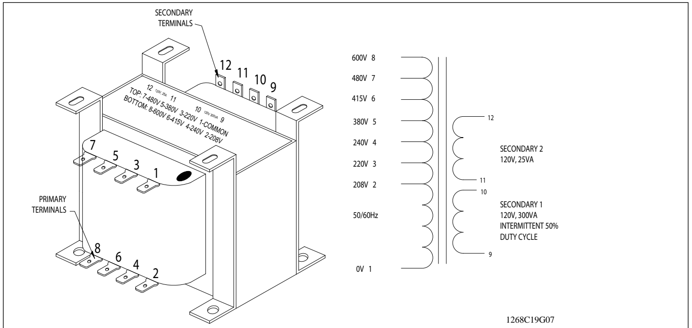
Figure 22. Transformer and Taps.
