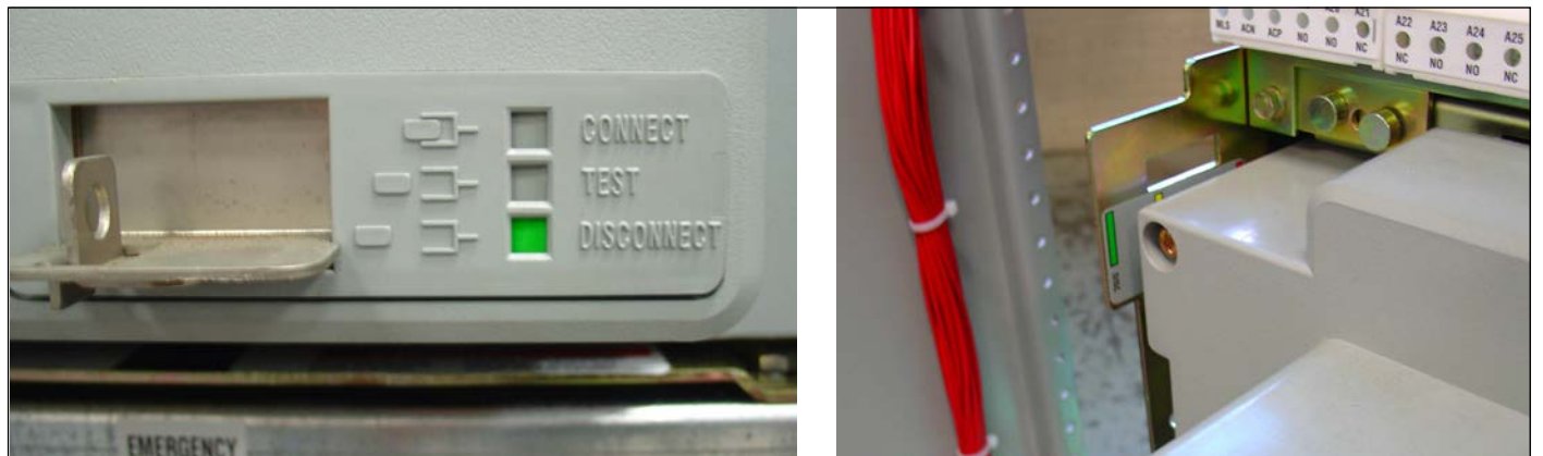
Figure 32. Switching Device in the DISCONNECT Position.
