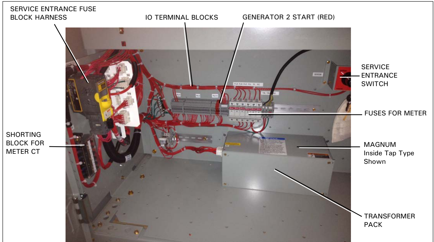
Figure 43. Bottom Panel for User Interface
