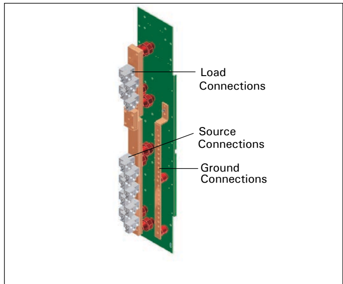
Figure 19. Solid Neutral.
