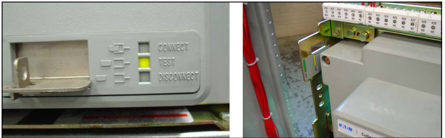
Figure 31. Switching Device in the TEST Position.
