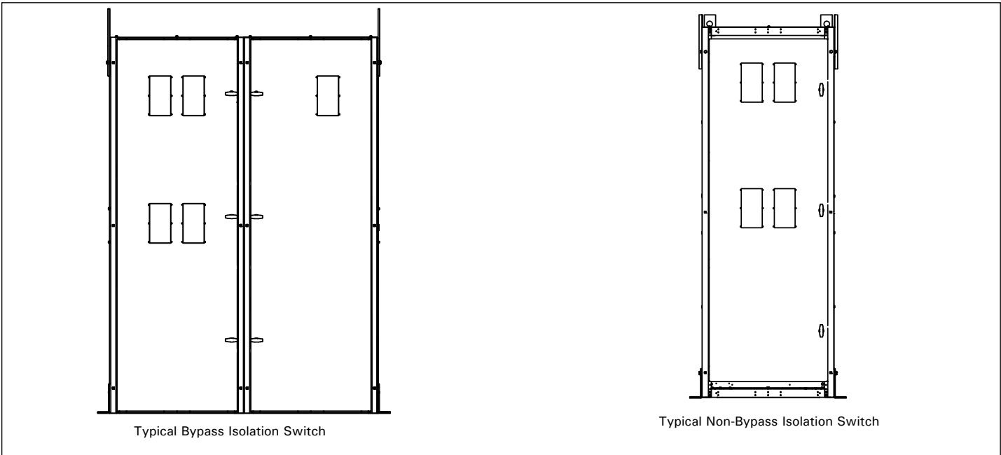
Figure 3. Typical Bypass Isolation Switch.
