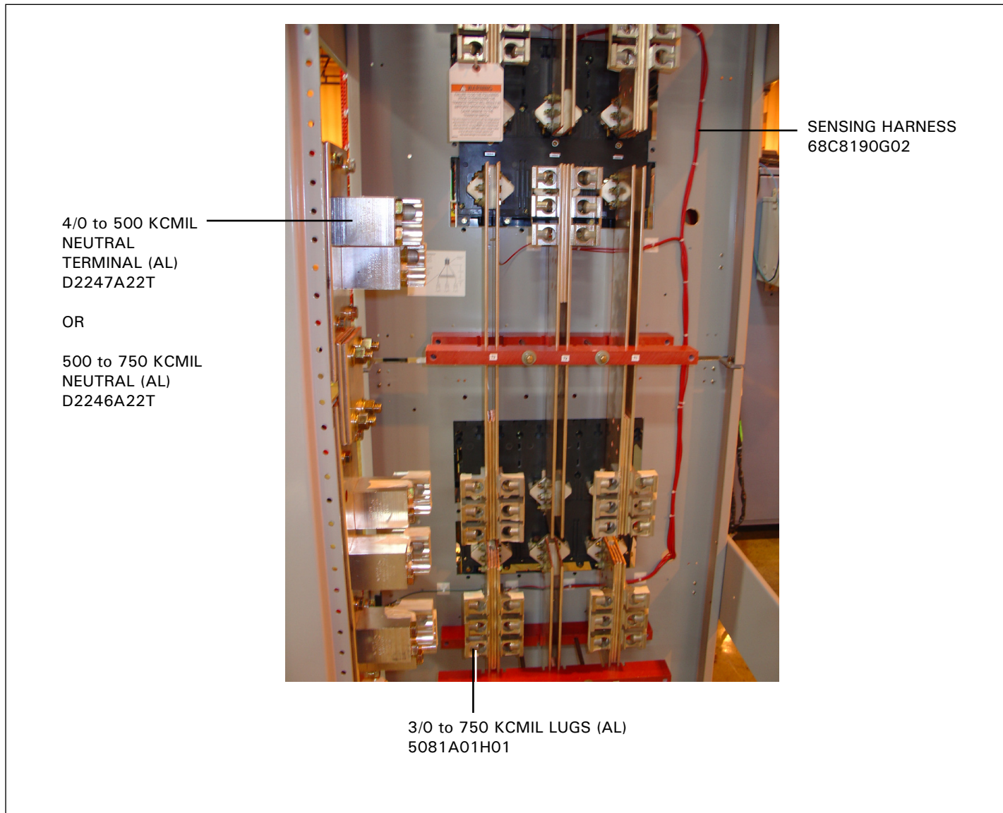
Figure 45. Rear of Switch
