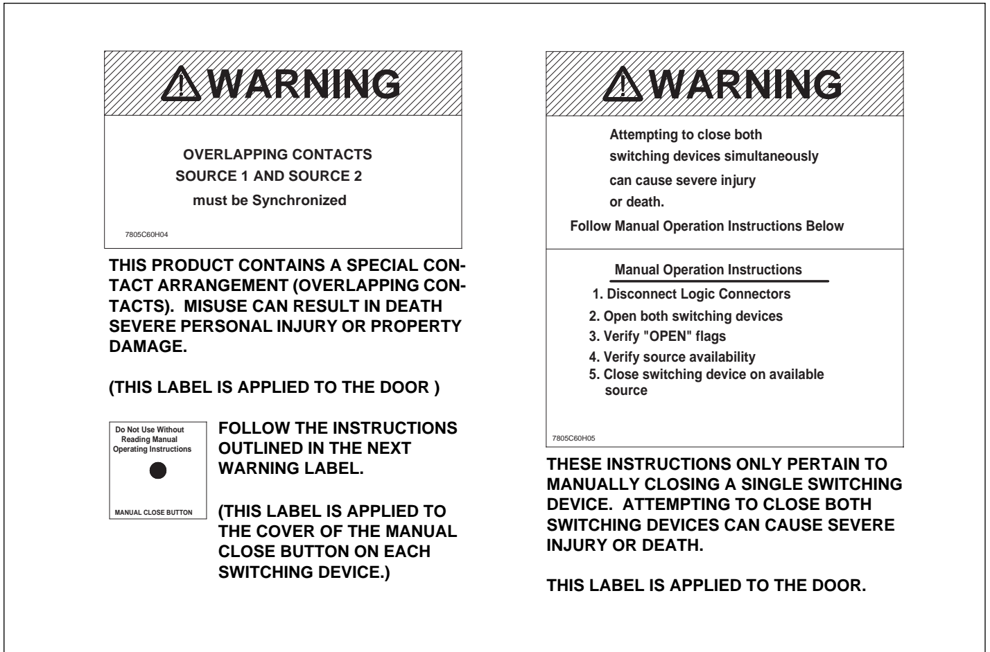
Figure 26. Switching Device Closing Precautions (Closed Transition Only).
