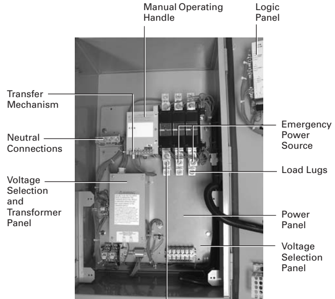
Typical Contactor-Based ATS 100 – 600 Amperes
