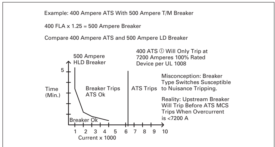
Figure 16-4. Built-in Protection
