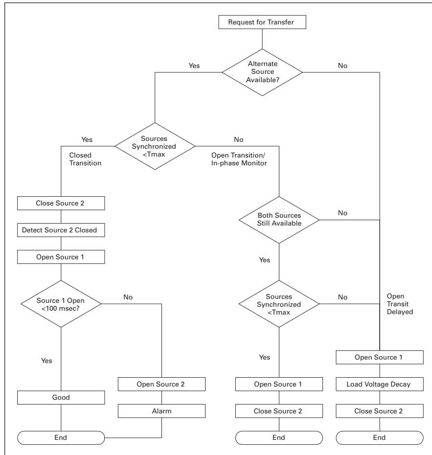
Figure 16-18. Feature Set 47C Schematic
