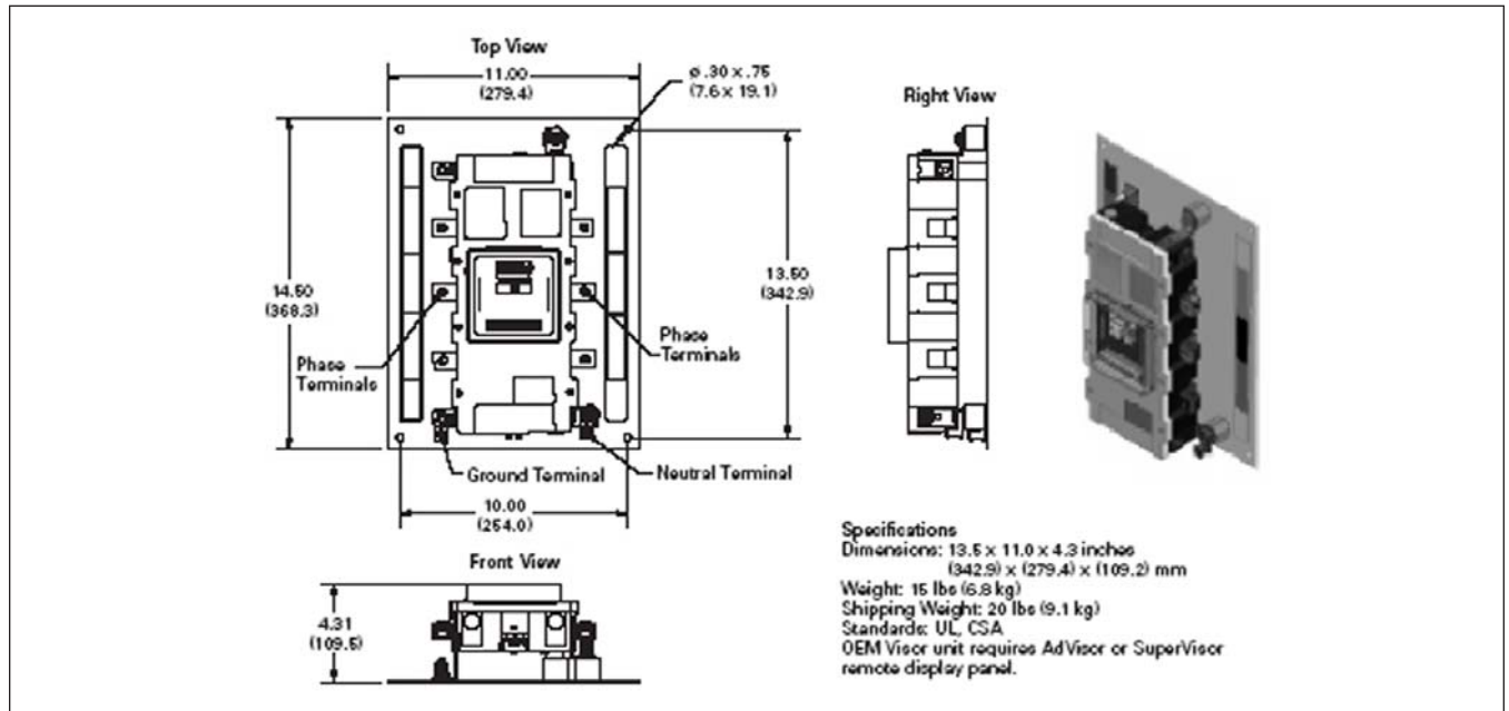
Figure 16-20. Visor OEM 100, 100 and 200 kA Technical Data
