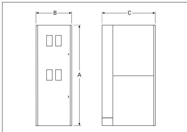
Figure 16-12. 200 – 2000 Ampere Fixed Mount NEMA 1
