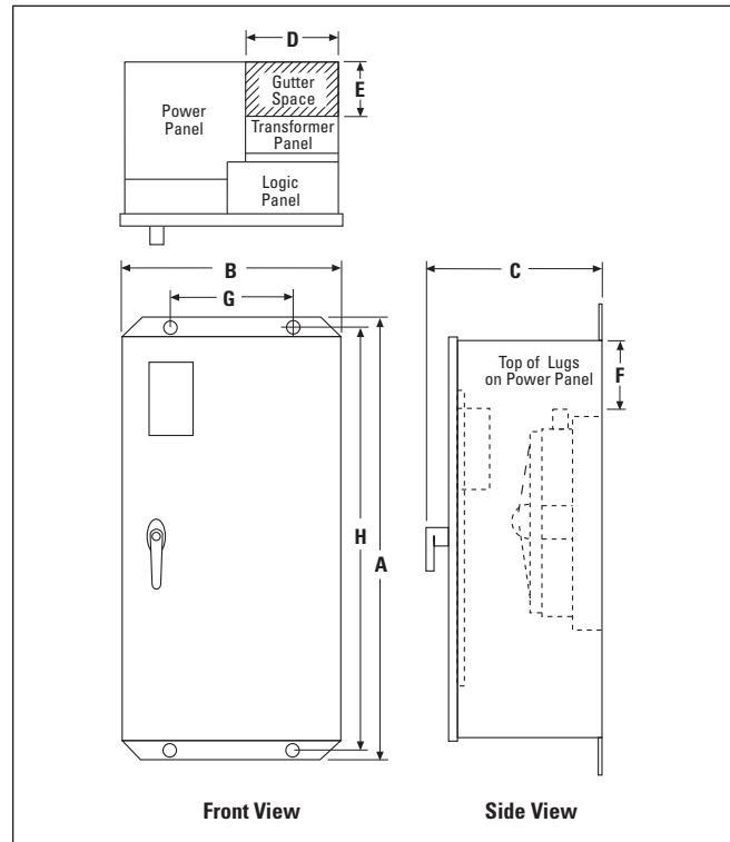
Figure 16-7. Dimensions
