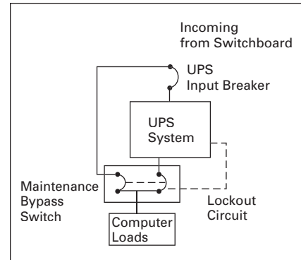
Figure 16-8. Single Line Diagram of Maintenance Bypass Switch
