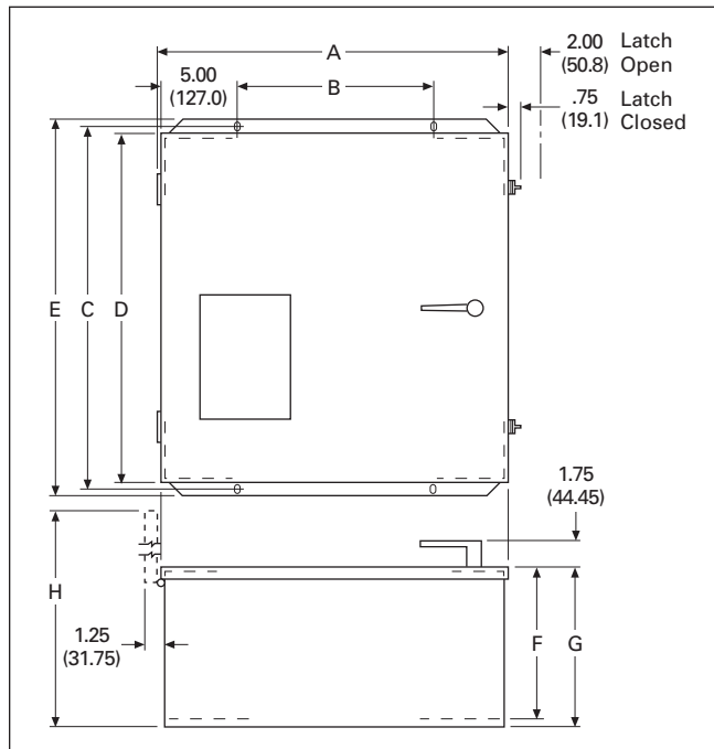
Figure 16-5. Dimensions
