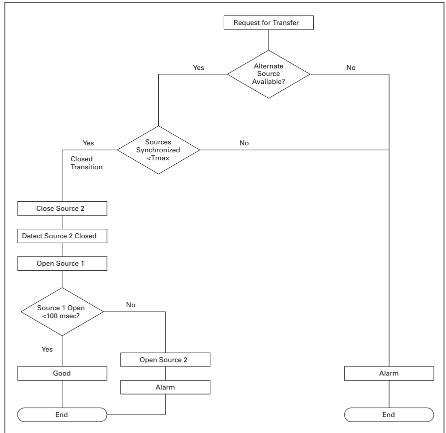
Figure 16-19. Feature Set 47D Schematic
