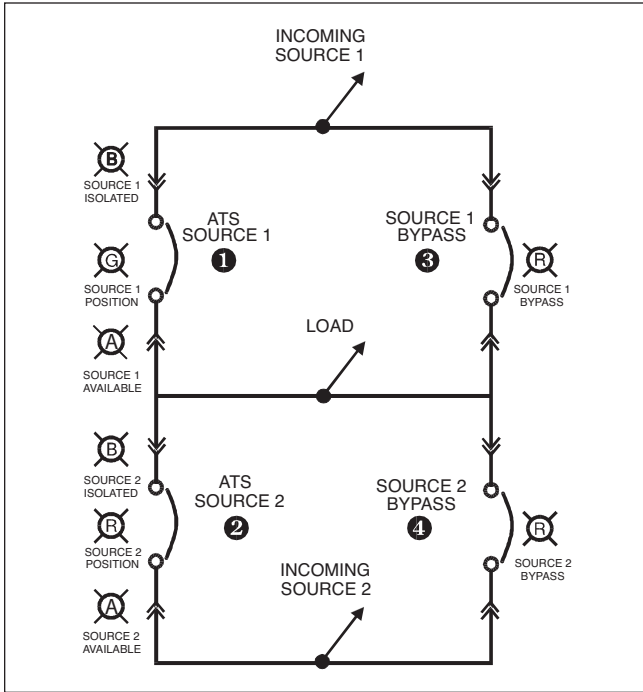
Figure 16-11. Typical Bypass Isolation Switch Schematic
