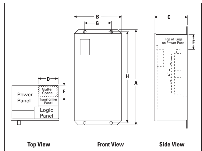
Figure 16-6. Dimensions
