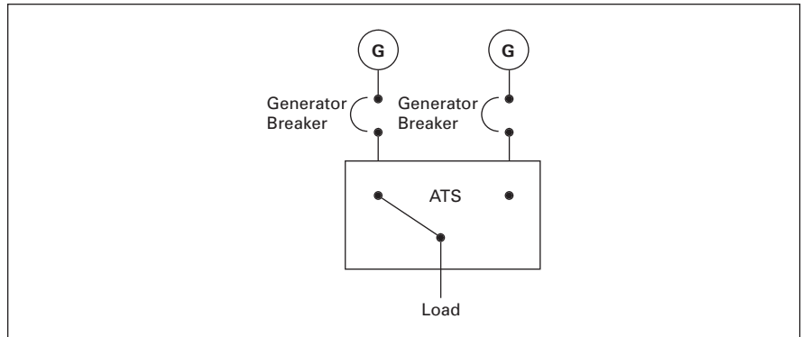
Figure 16-2. Standard Application Generator — Generator
