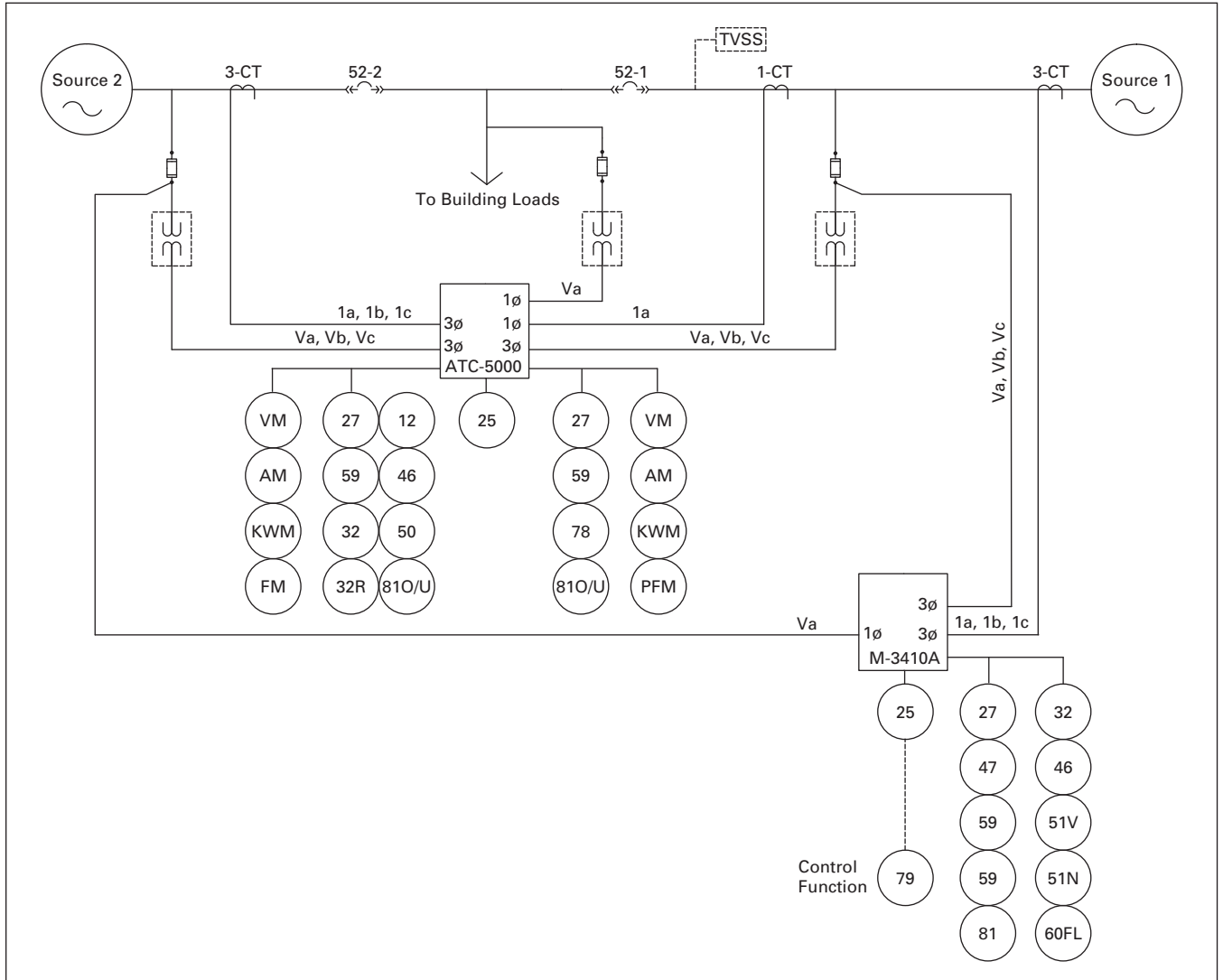
Figure 16-24. Typical System Diagram — Standard One Line With Utility Grade Multi-function Relaying
