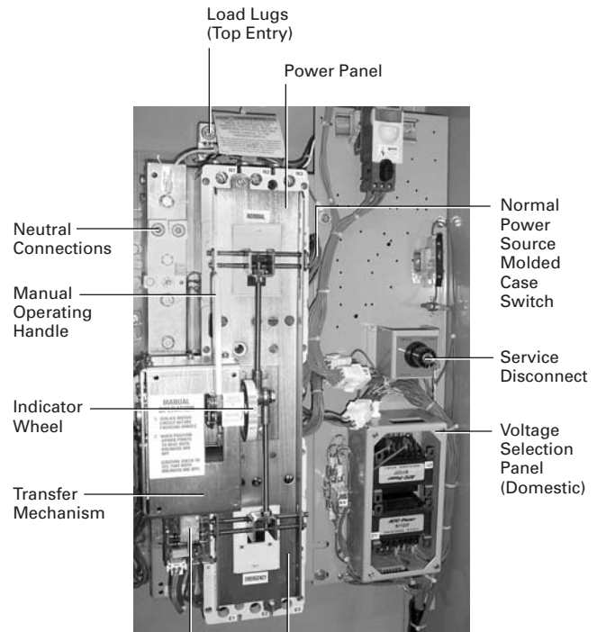
Typical Contactor-Based ATS 100 – 600 Amperes
