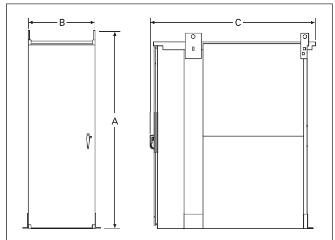
Figure 16-17. 200 – 2000 Ampere Drawout NEMA 3R
