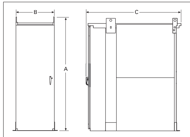
Figure 16-15. 200 – 2000 Ampere Drawout NEMA 3R
