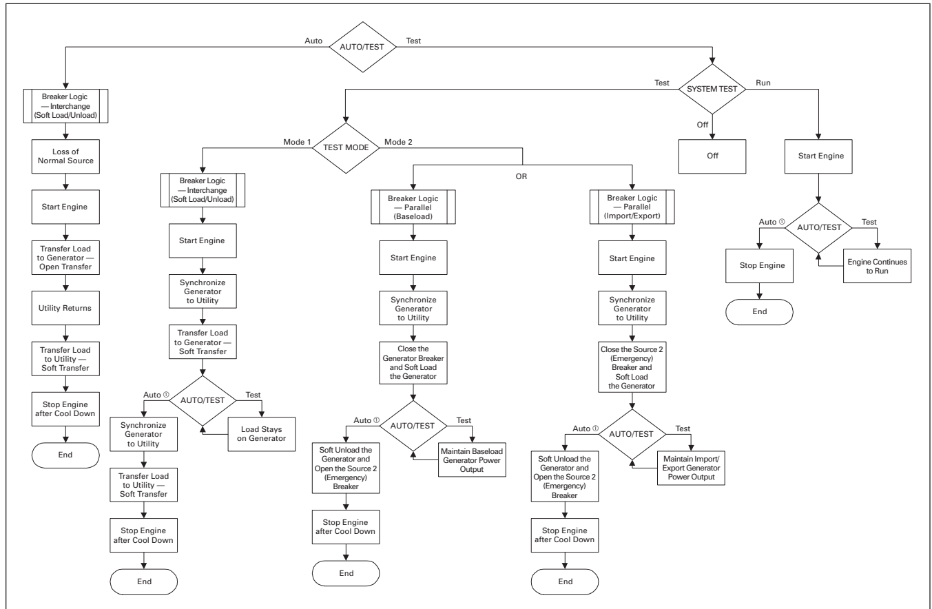
Figure 16-22. Sequence Flow Chart — Soft Load ATS with Extended Paralleling Capabilities
