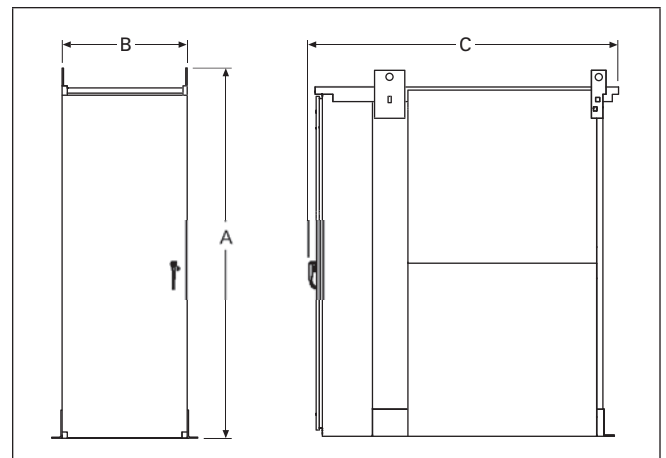
Figure 16-13. 200 – 2000 Ampere Fixed Mount NEMA 3R
