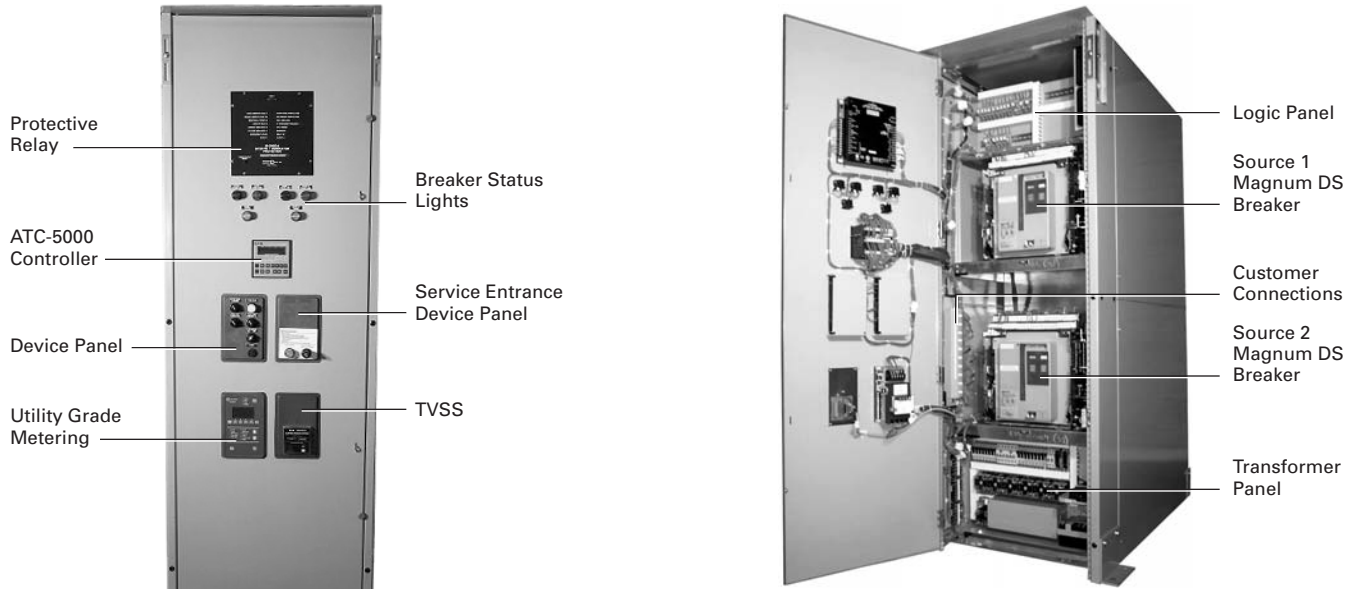
Magnum Soft Load ATS Base Components
