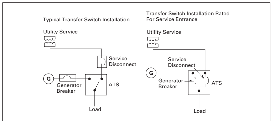
Figure 16-3. Service Entrance Rated Transfer Switches
