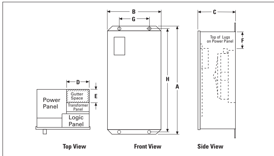
Figure 16-10. Dimension Views
