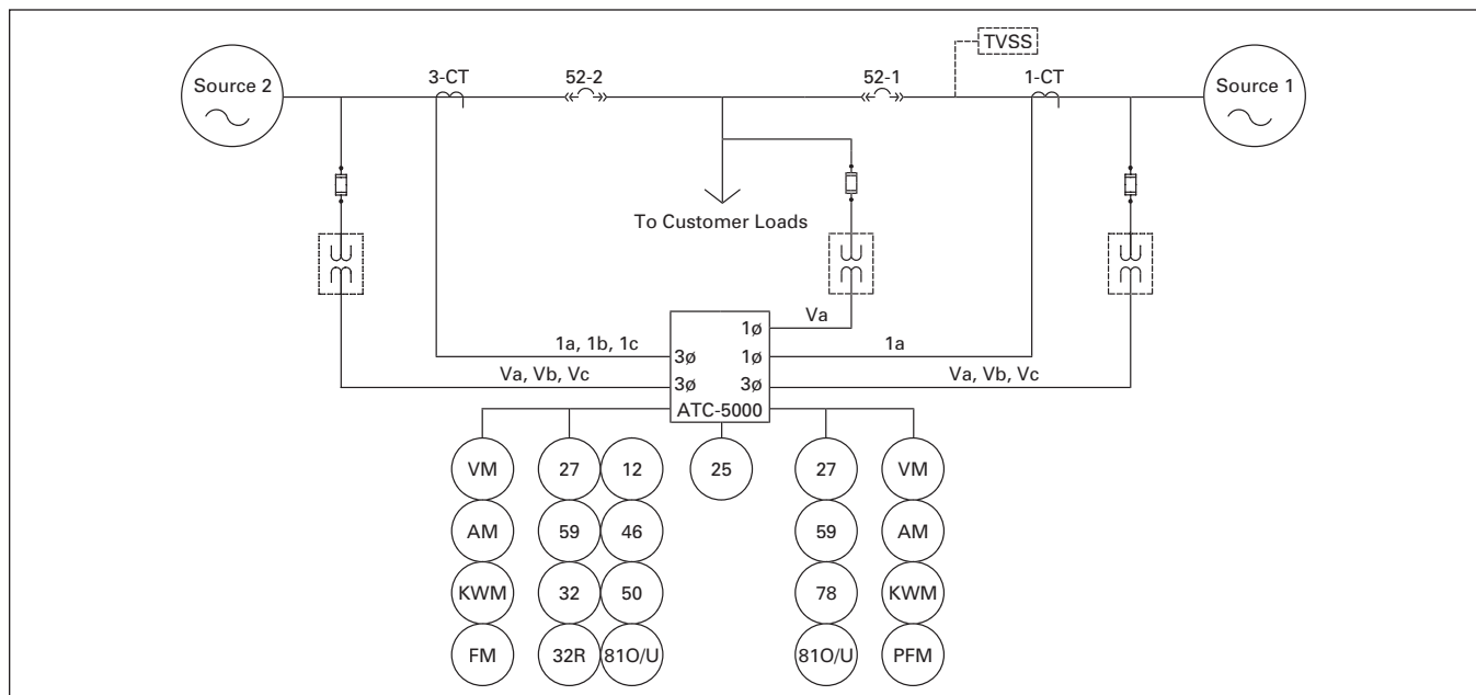
Figure 16-23. Typical System Diagram — Standard One Line
