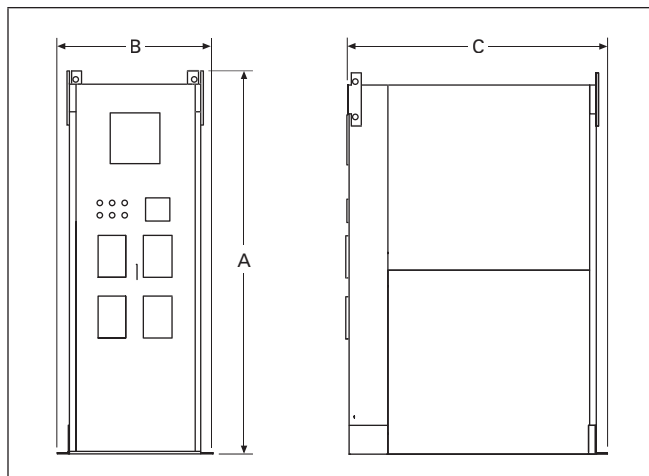
Figure 16-16. 200 – 2000 Ampere Drawout NEMA 1
