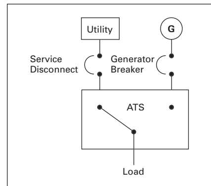
Figure 16-1. Standard Application Utility — Generator
