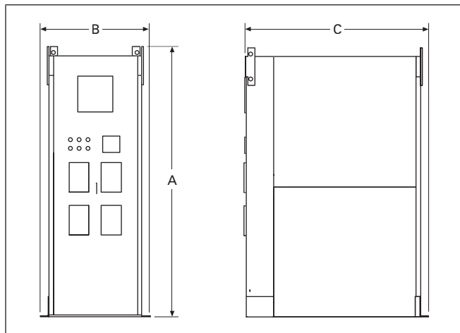
Figure 16-14. 200 – 2000 Ampere Drawout NEMA 1
