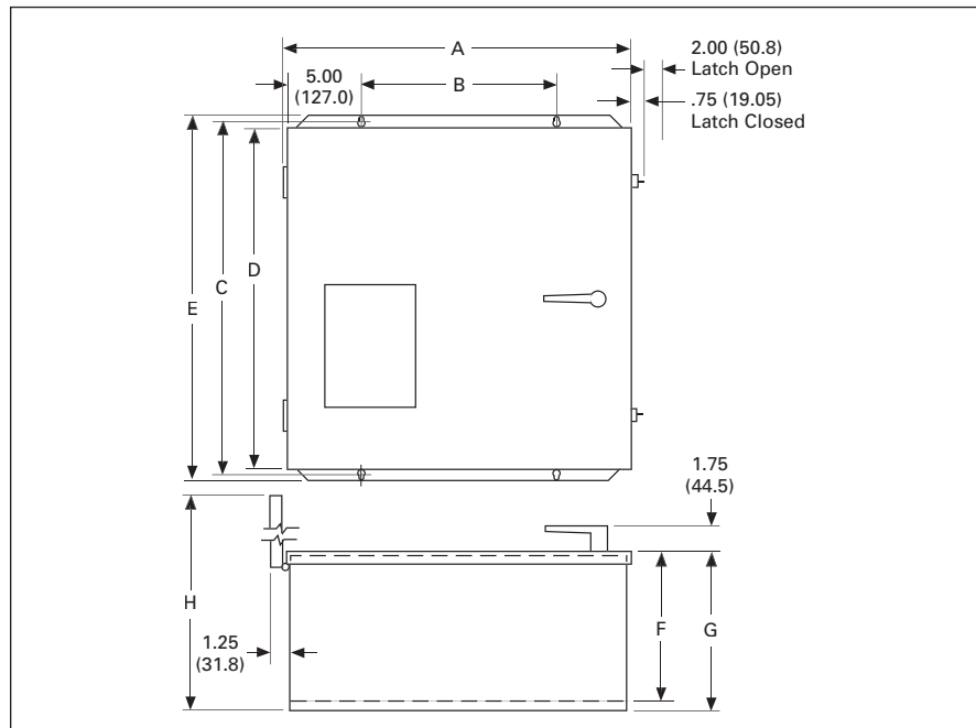
Figure 16-9. Manual and Maintenance Bypass Switches — Dimensions in Inches (mm)
