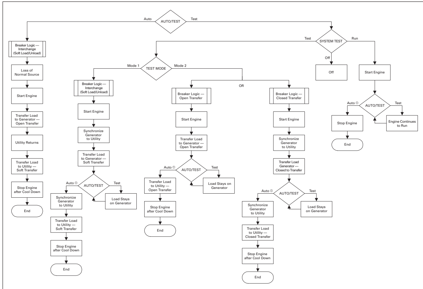
Figure 16-21. Sequence Flow Chart — Soft Load ATS
