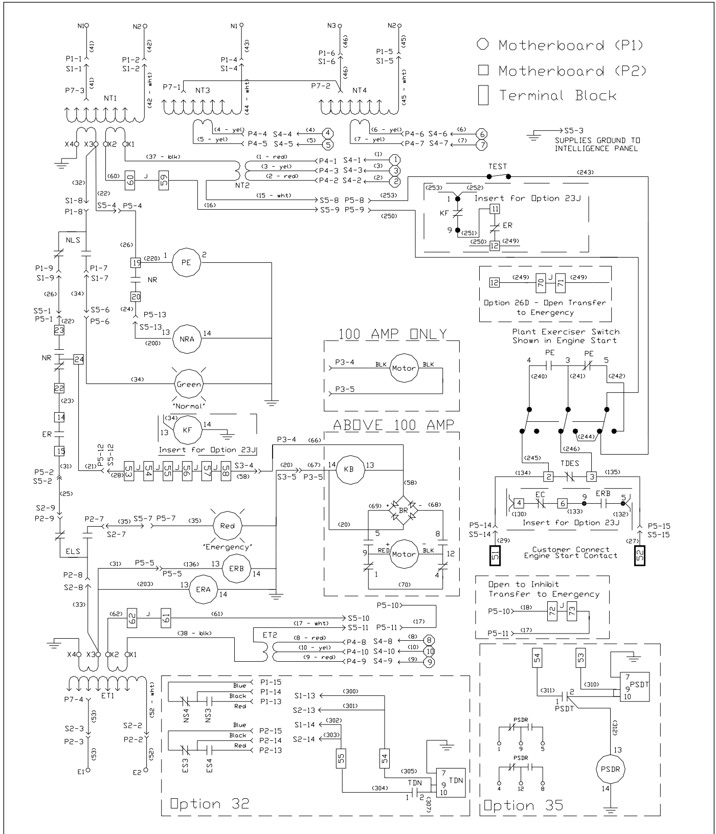
Figure 8-1 Wiring Diagram for AGswitch Automatic Transfer Switch
