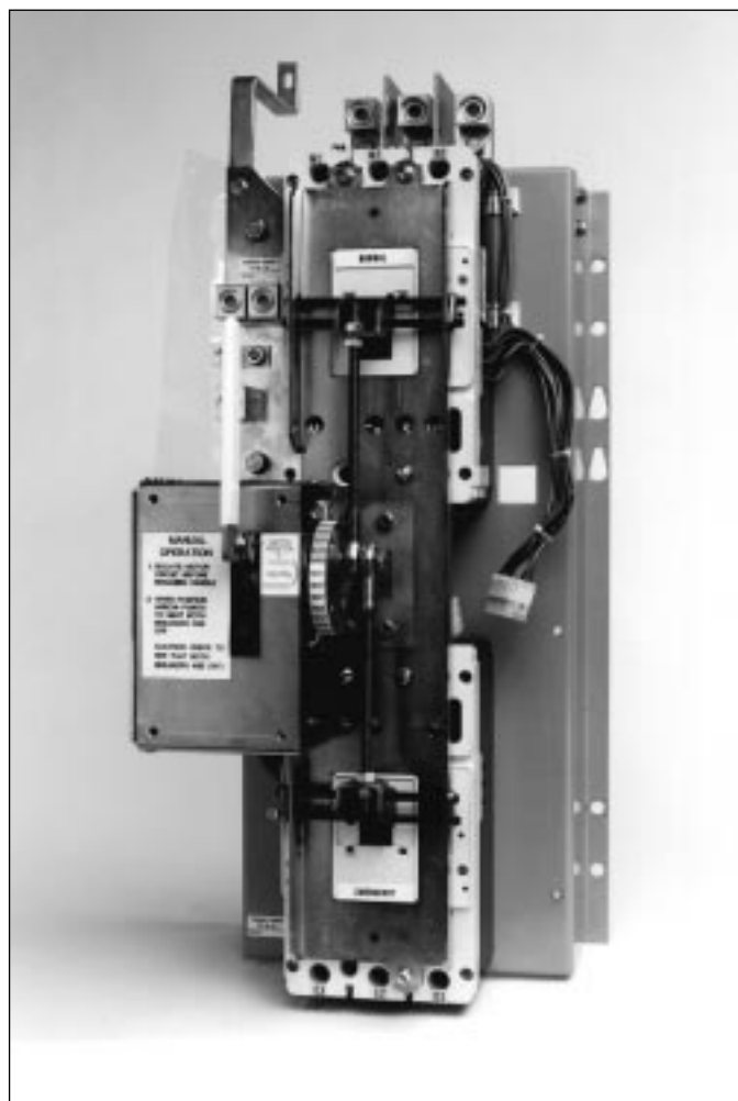
Figure 3-1 Typical Power Panel (Unmounted) for 225-1000A Models
