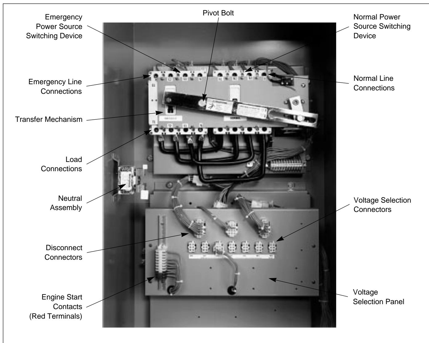
Figure 4-2 Typical (30-150 Amperes) Horizontal Design Transfer Switch Equipment (Door Open)
