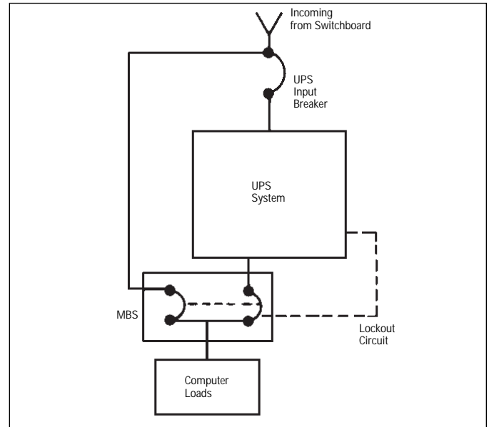
Figure 1 Application with Static UPS System
