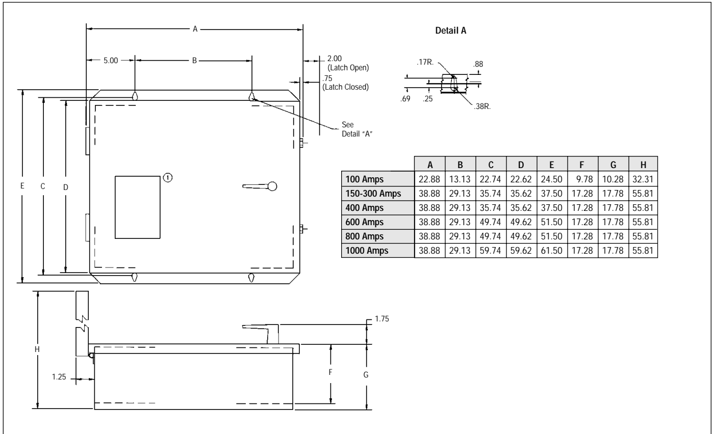
Figure 2 Outline Dimensions
