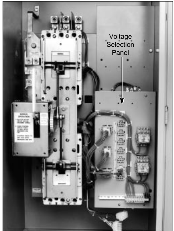
Figure 1-3 Vertical Design Automatic Transfer Switch Equipment Shown with Deadfront Cover Removed (225-1000 Amperes)
