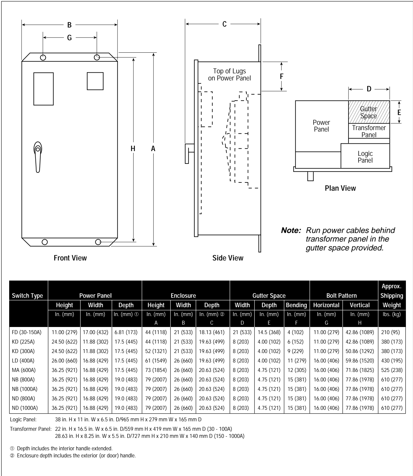
Figure 4-1 Enclosed Automatic Transfer Switch Dimensions and Approximate Weights
