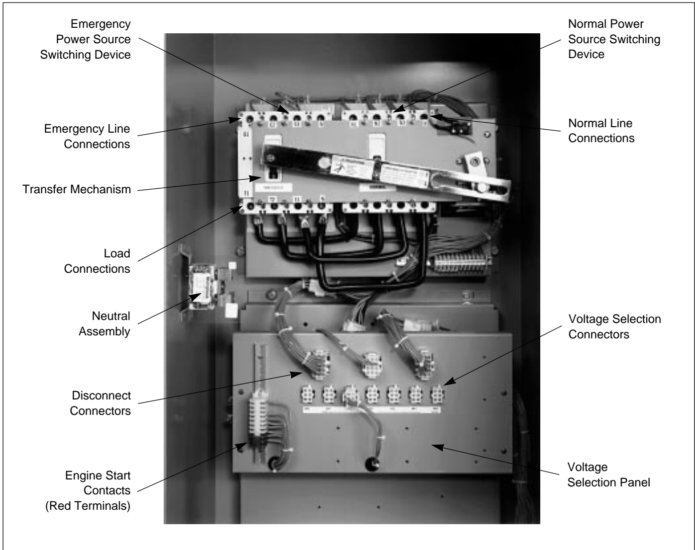
Figure 4-5 Typical (30-150 Amperes) Horizontal Design Transfer Switch Equipment (Door Open)
