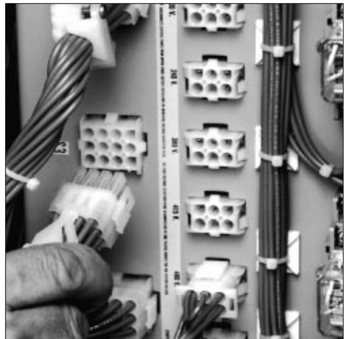
Figure 5-4 Motor Disconnect Being Unplugged
