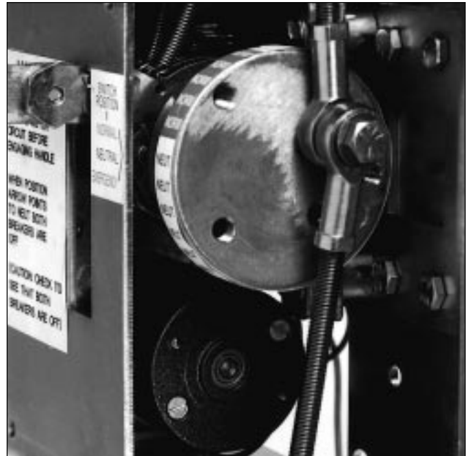
Figure 5-2 Indicator Wheel Shown Mounted in Mechanism with Motor Mounted Under Wheel
