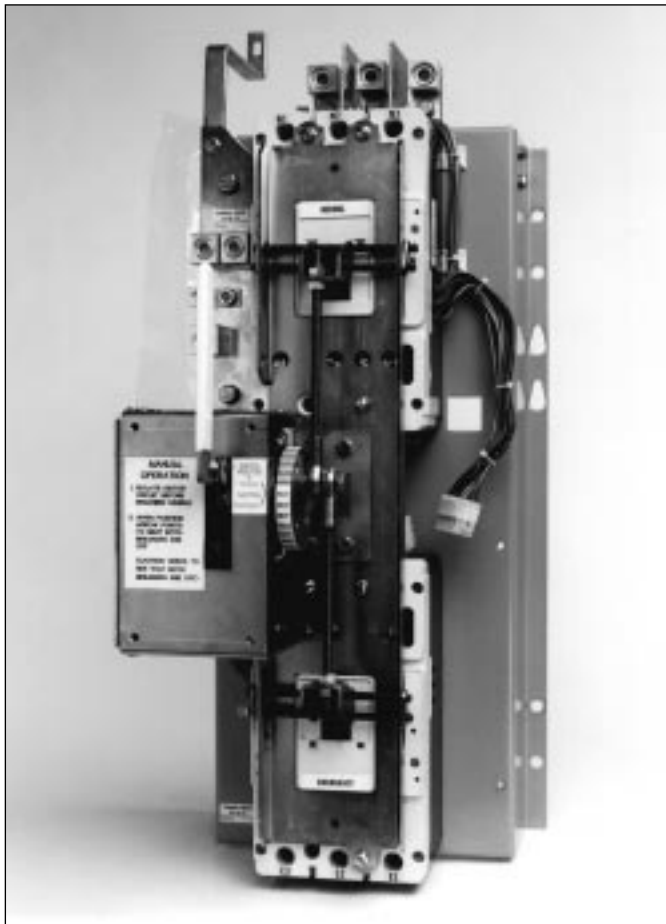
Figure 3-1 Typical Vertical Design Power Panel (Unmounted)
