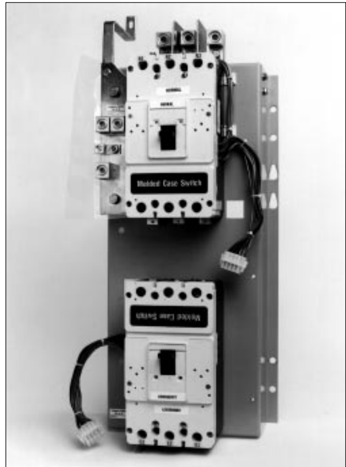
Figure 3-3 Molded Case Switches Mounted in Vertical Design (Transfer Mechanism Removed for Clarity)
