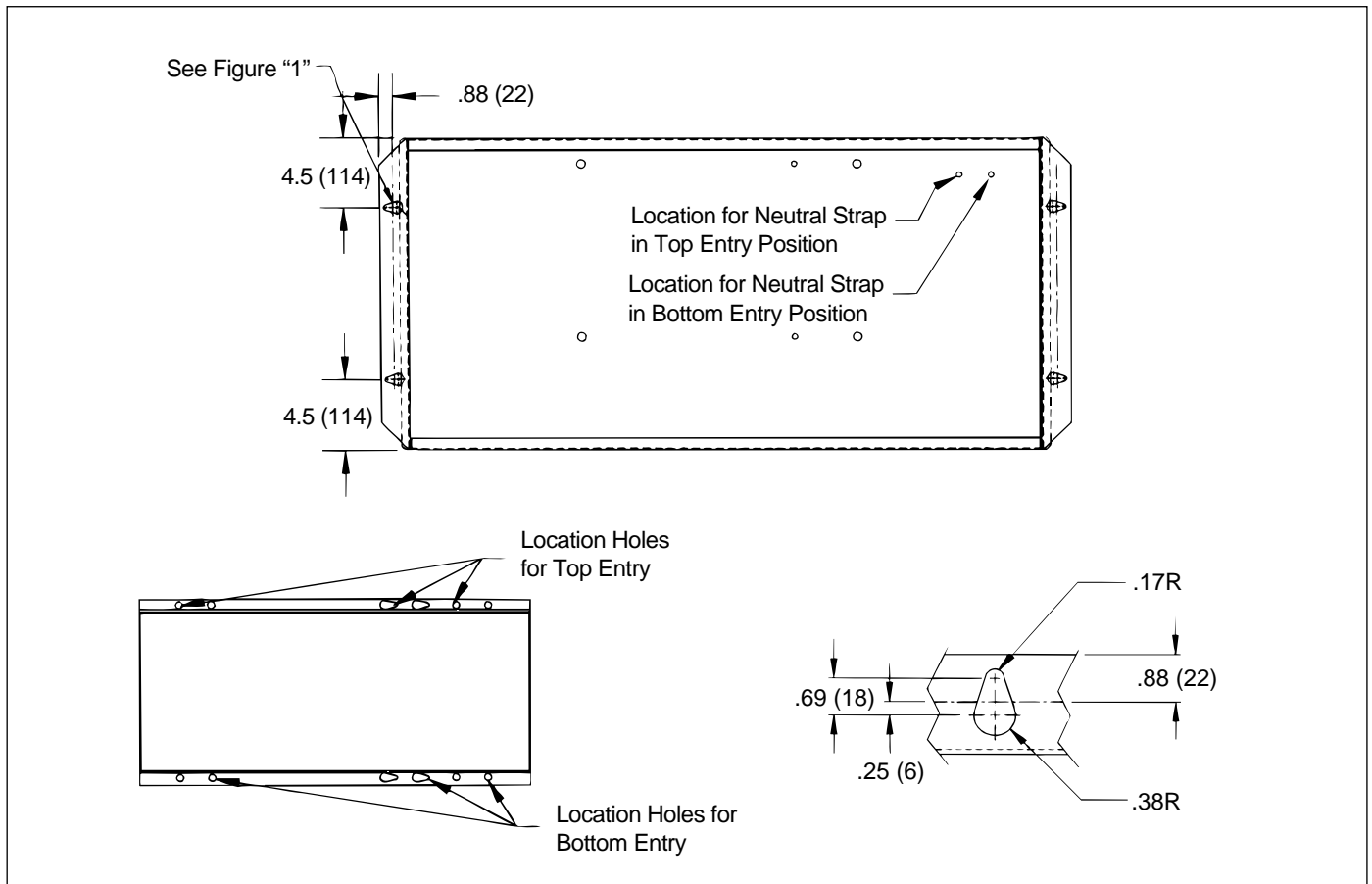
Figure 4-2 Vertical Design Power Panel Mounting Reference in Inches (mm)
