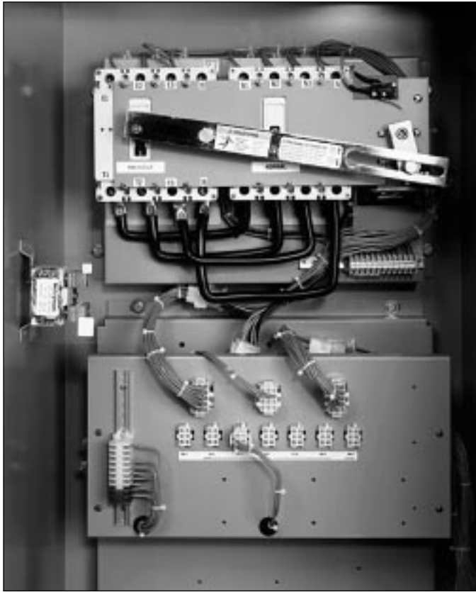
Figure 1-4 Horizontal Design Automatic Transfer Switch Equipment (30-150 Amperes)
