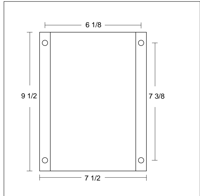
Figure 3-6 Charger Mounting Dimensions in inches (mm)
