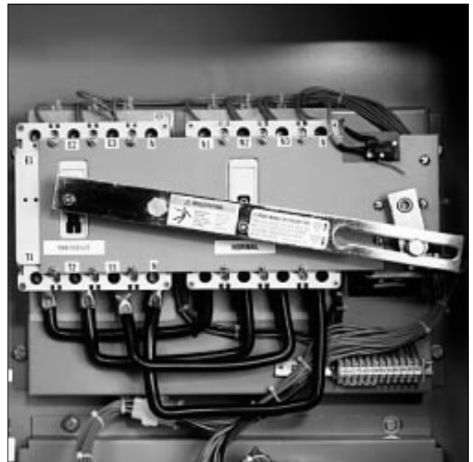
Figure 3-2 Typical Horizontal Design Power Panel (Mounted)
