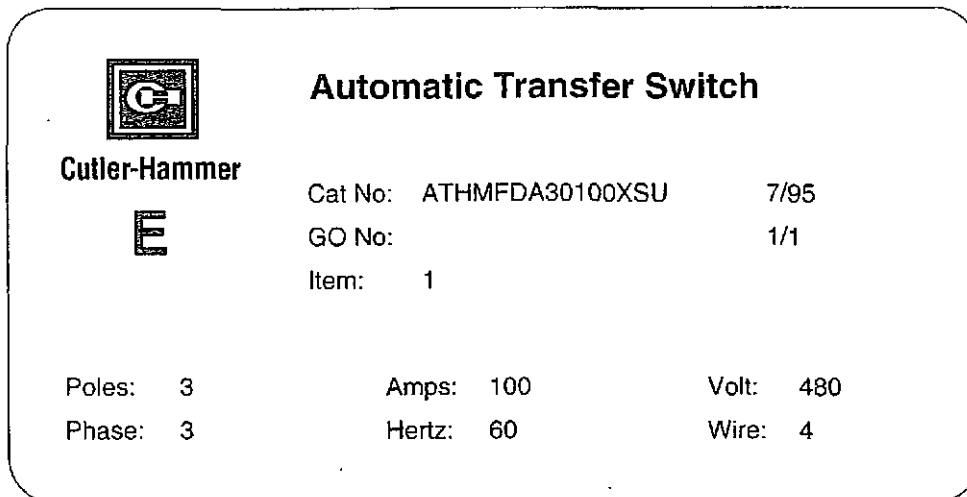
Figure 1 Typical Automatic Transfer Switch Equipment Nameplate
