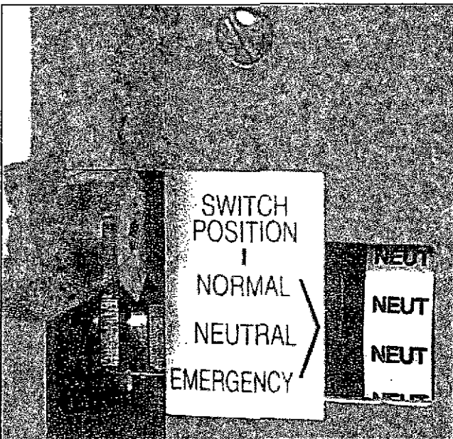
Figure 5-4 Indicator Wheel in Neutral Position (225-1000A Models)
