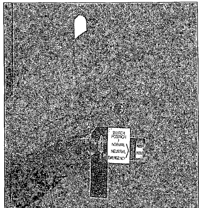
Figure 5-2 Transfer Switch Manual Operating Handle in Use (225-1000A Models)
