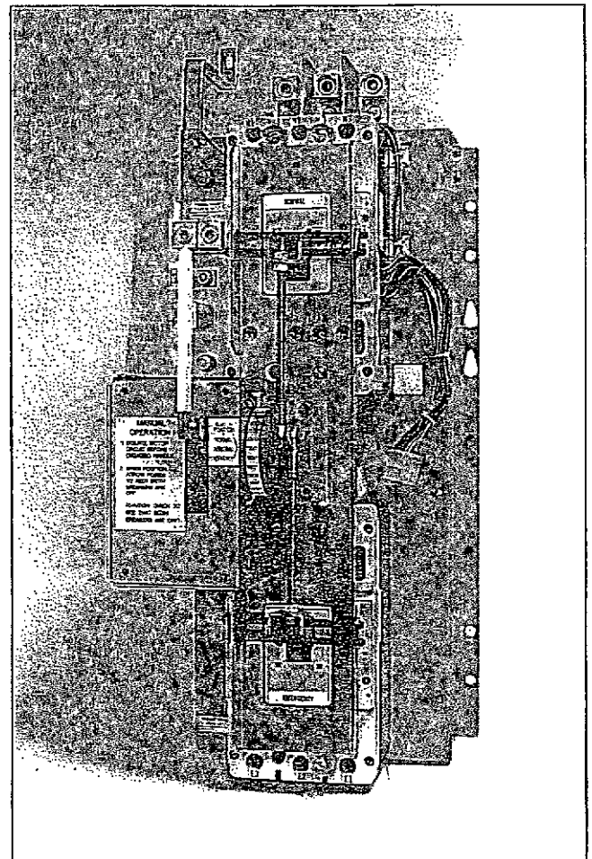
Figure 3-1 Typical Power Panel (Unmounted) for 225-1000A Models
