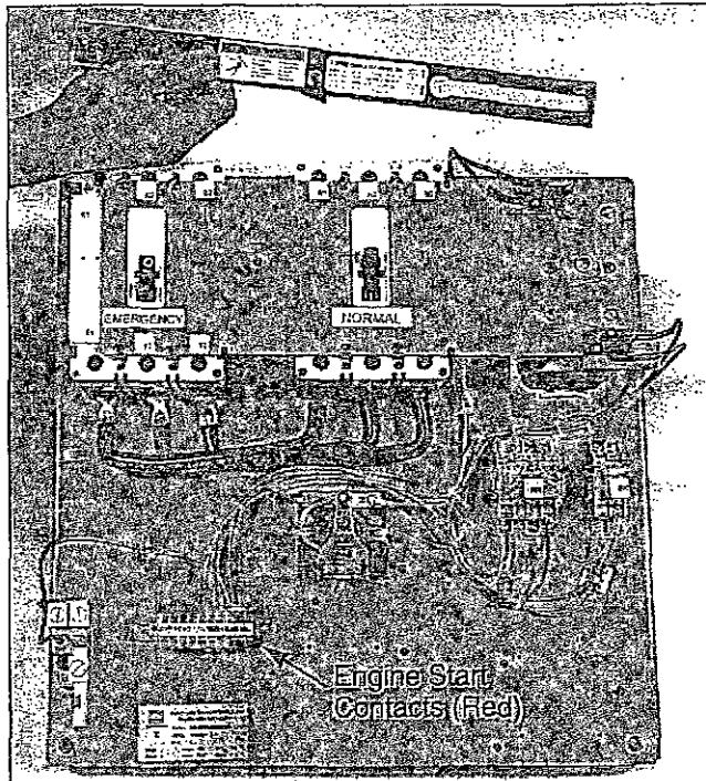
Figure 5-5 Transfer Mechanism with Lever Removed (30-150A Model)
