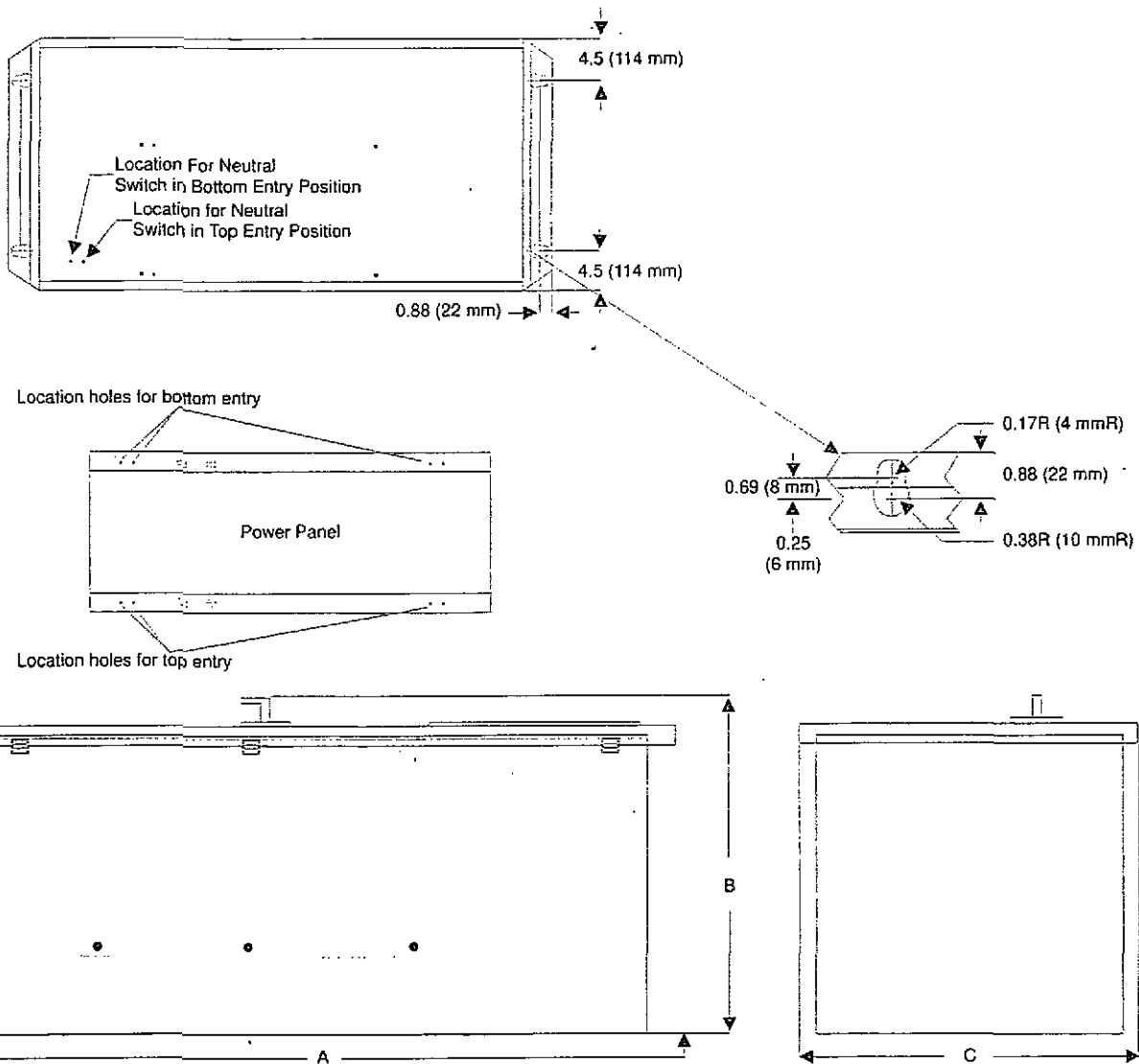
Figure 4-1 Dimensions of Enclosed Automatic Transfer Switch and Approximate Weights
