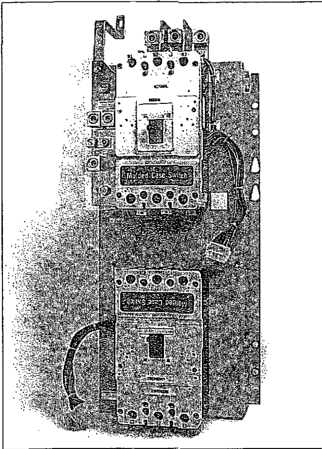
Figure 3-3 Mounted Molded Case Switches with the Transfer Mechanism Removed for Clarity (225-1000A Models)
