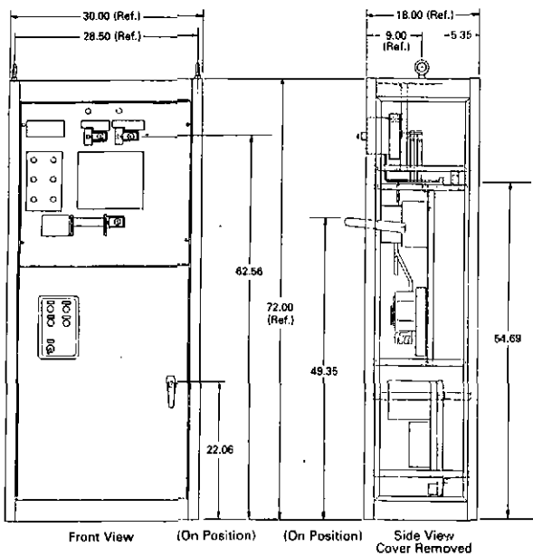
ENCLOSURE DIMENSIONS 100 AMPS
