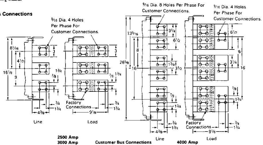
Figure 1 Reproduced From Drawing 1375D51
