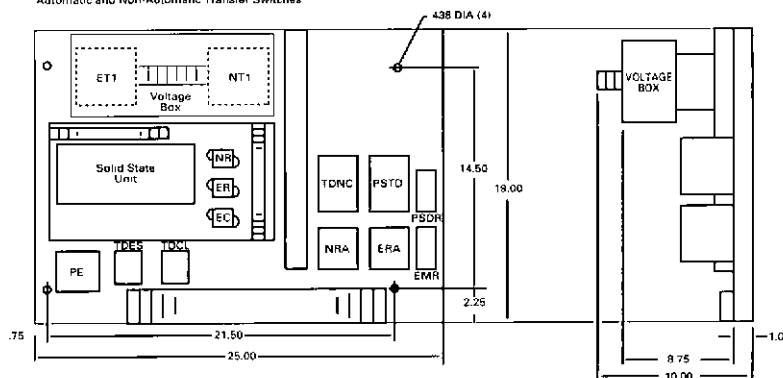
Solid State Logic Panel - 100-1000 Amperes, 2, 3, 4, Poles Automatic and Non-Automatic Transfer Switches
