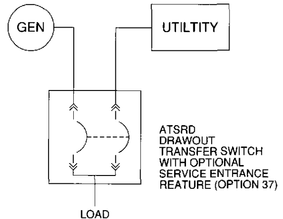
Fig. 2. Service Entrance Transfer Switch
