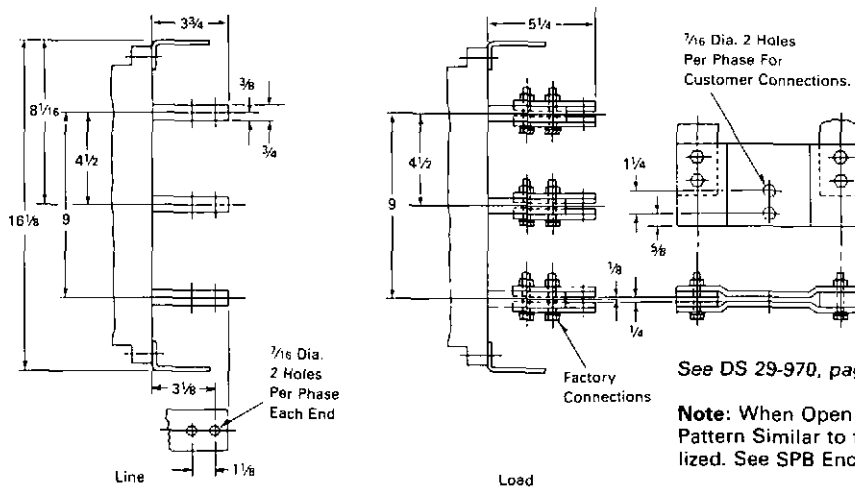
Figure 1 Reproduced From Drawing 1375D52
