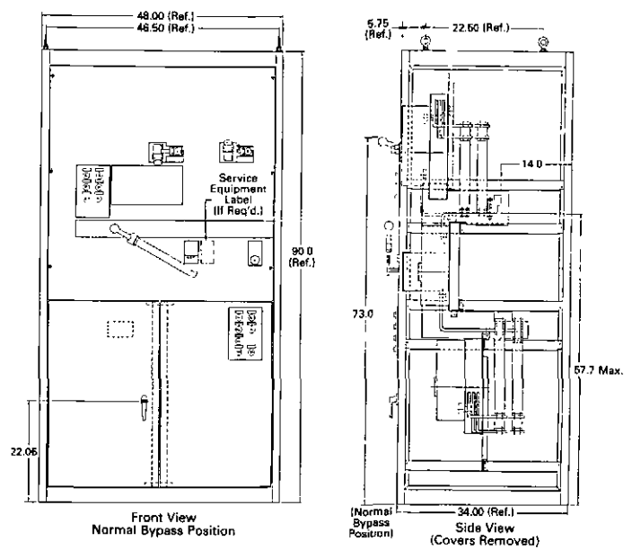
ENCLOSURE DIMENSIONS 150-1000 AMPS
