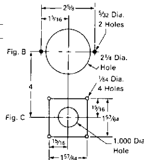
Figure 2 Reproduced From Drawings 1370D19, 751B655
