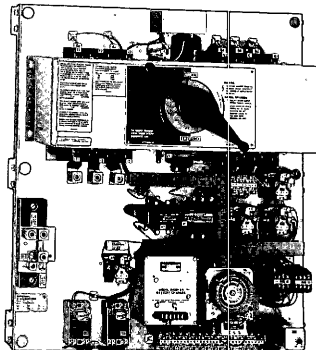
Open Transfer Switch
