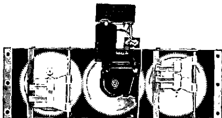
Rearview, Transfer Mechanism, 150-400 Ampere Switches
