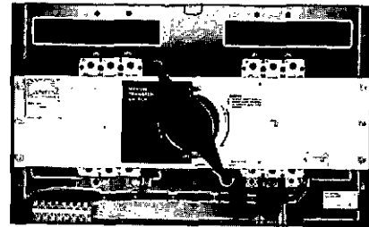
Single Handle Manual Transfer Switch — Type MTSSM
