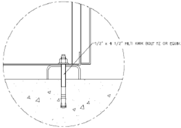
TYP. FLOOR ANCHORING
